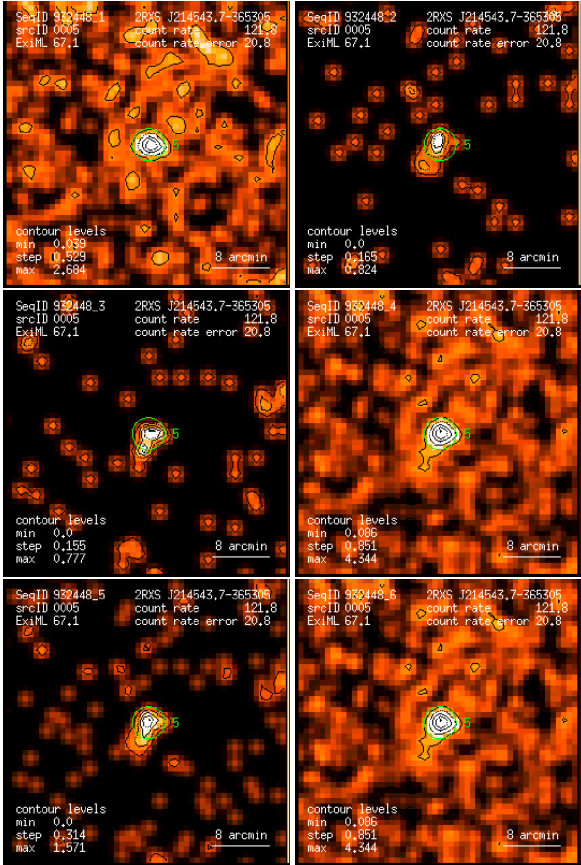
Figure 5: RASS 932448: detection 0005: band rate images, Gaussian filter: (1) PSPC channels 11 – 41, (2) 52 – 90, (3) 91 – 201, (4) 11 – 235, (5) 52 – 201, (6) 11 – 201. Broad band rates in counts/ks. Band rate contour levels in counts/ks/arcmin 2 .
