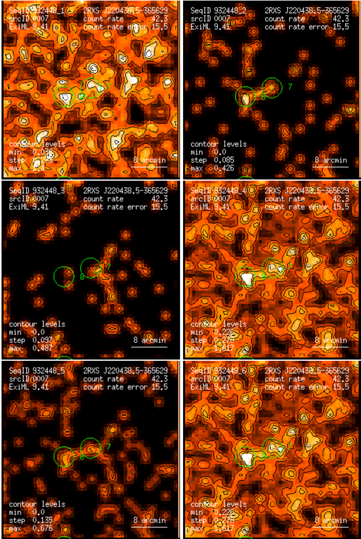
Figure 7: RASS 932448: detection 0007: band rate images, Gaussian filter: (1) PSPC channels 11 – 41, (2) 52 – 90, (3) 91 – 201, (4) 11 – 235, (5) 52 – 201, (6) 11 – 201. Broad band rates in counts/ks. Band rate contour levels in counts/ks/arcmin 2 .
