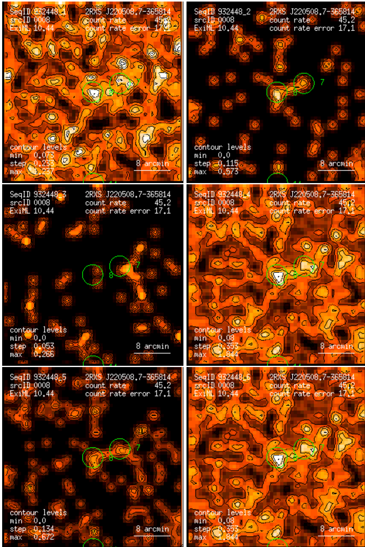
Figure 8: RASS 932448: detection 0008: band rate images, Gaussian filter: (1) PSPC channels 11 – 41, (2) 52 – 90, (3) 91 – 201, (4) 11 – 235, (5) 52 – 201, (6) 11 – 201. Broad band rates in counts/ks. Band rate contour levels in counts/ks/arcmin 2 .
