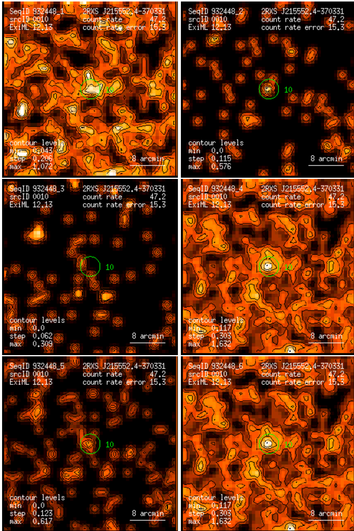
Figure 10: RASS 932448: detection 0010: band rate images, Gaussian filter: (1) PSPC channels 11 – 41, (2) 52 – 90, (3) 91 – 201, (4) 11 – 235, (5) 52 – 201, (6) 11 – 201. Broad band rates in counts/ks. Band rate contour levels in counts/ks/arcmin 2 .
