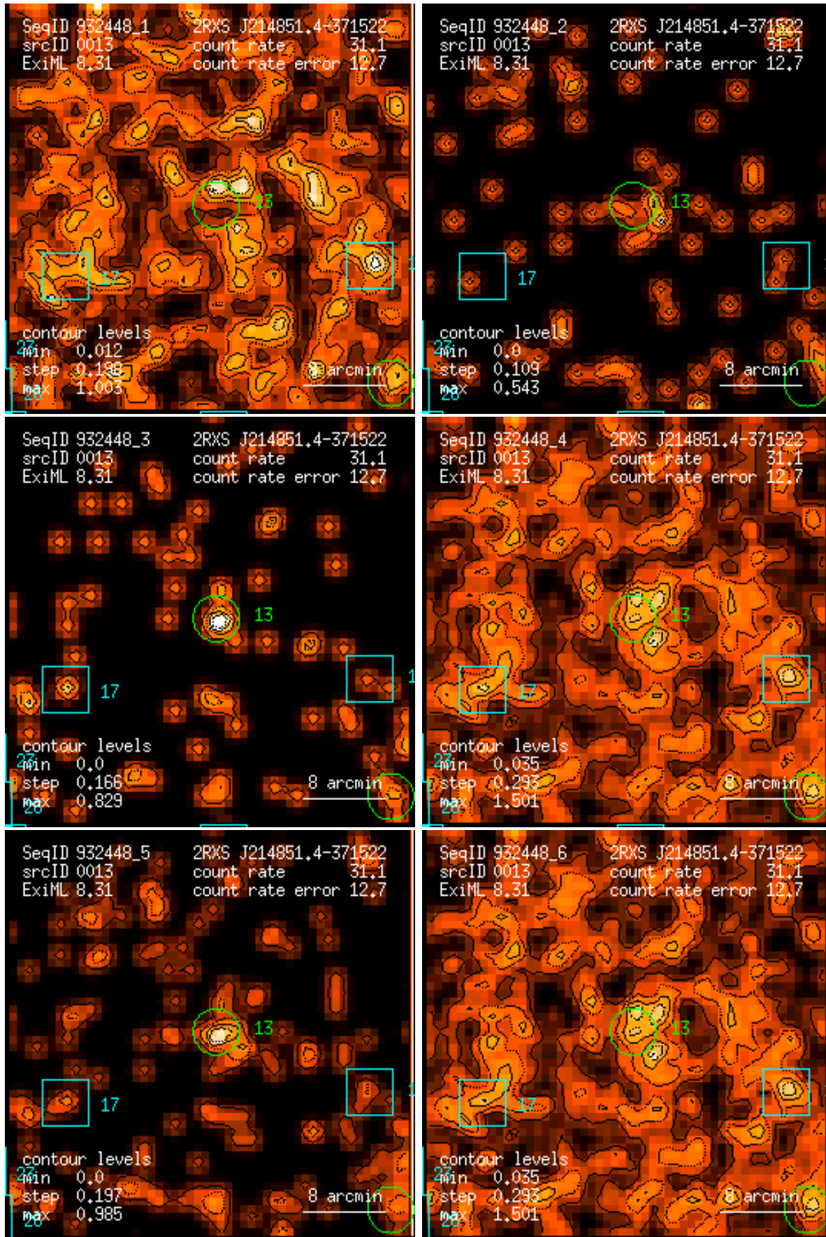
Figure 13: RASS 932448: detection 0013: band rate images, Gaussian filter: (1) PSPC channels 11 – 41, (2) 52 – 90, (3) 91 – 201, (4) 11 – 235, (5) 52 – 201, (6) 11 – 201. Broad band rates in counts/ks. Band rate contour levels in counts/ks/arcmin 2 .
