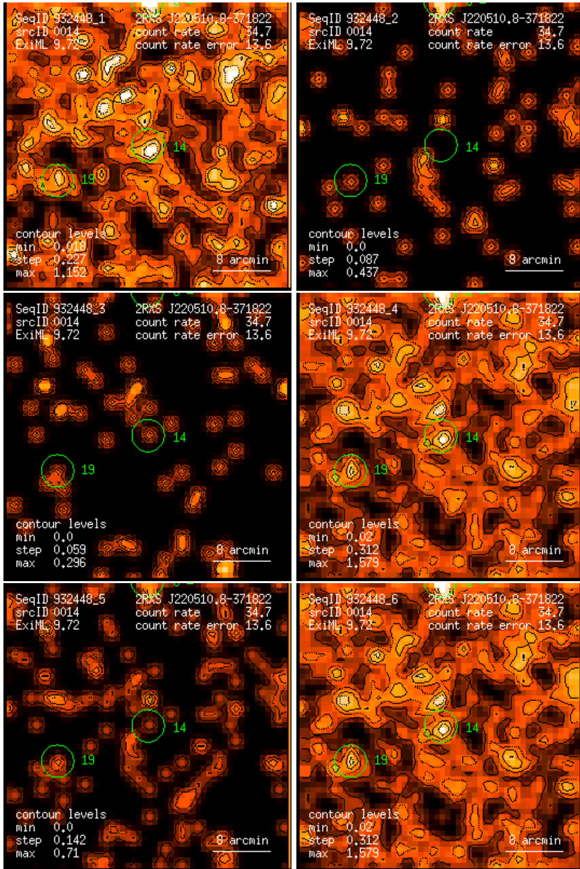
Figure 14: RASS 932448: detection 0014: band rate images, Gaussian filter: (1) PSPC channels 11 – 41, (2) 52 – 90, (3) 91 – 201, (4) 11 – 235, (5) 52 – 201, (6) 11 – 201. Broad band rates in counts/ks. Band rate contour levels in counts/ks/arcmin 2 .
