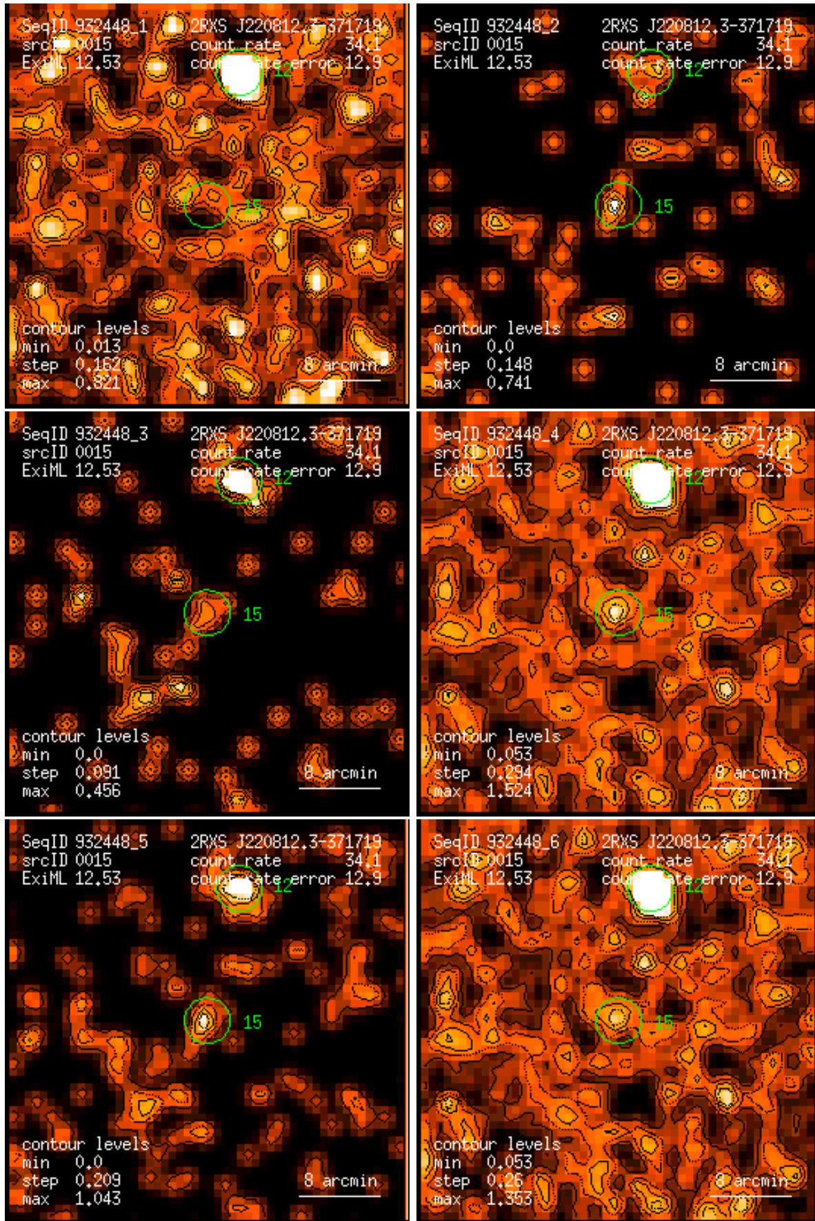
Figure 15: RASS 932448: detection 0015: band rate images, Gaussian filter: (1) PSPC channels 11 – 41, (2) 52 – 90, (3) 91 – 201, (4) 11 – 235, (5) 52 – 201, (6) 11 – 201. Broad band rates in counts/ks. Band rate contour levels in counts/ks/arcmin 2 .
