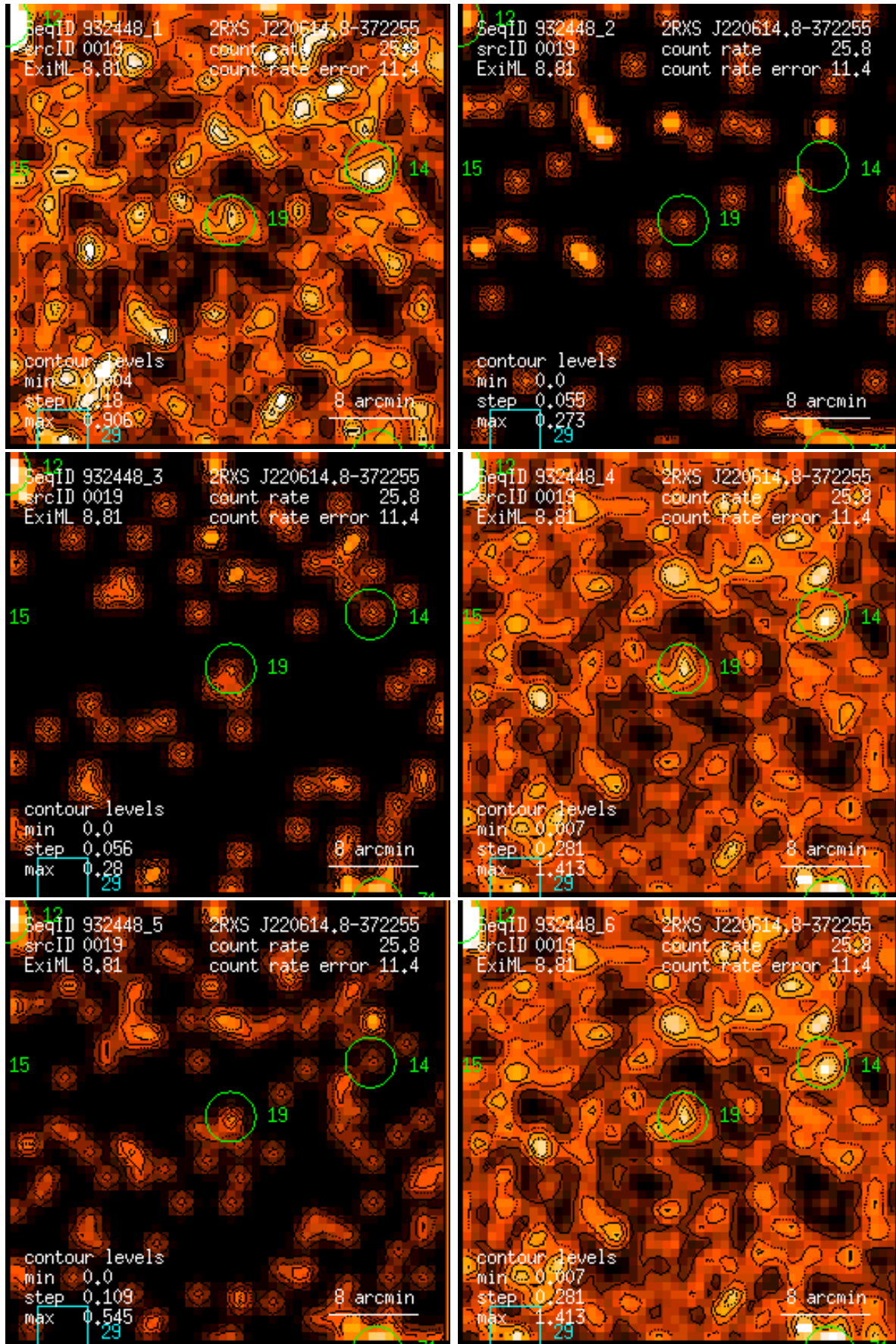
Figure 19: RASS 932448: detection 0019: band rate images, Gaussian filter: (1) PSPC channels 11 – 41, (2) 52 – 90, (3) 91 – 201, (4) 11 – 235, (5) 52 – 201, (6) 11 – 201. Broad band rates in counts/ks. Band rate contour levels in counts/ks/arcmin 2 .
