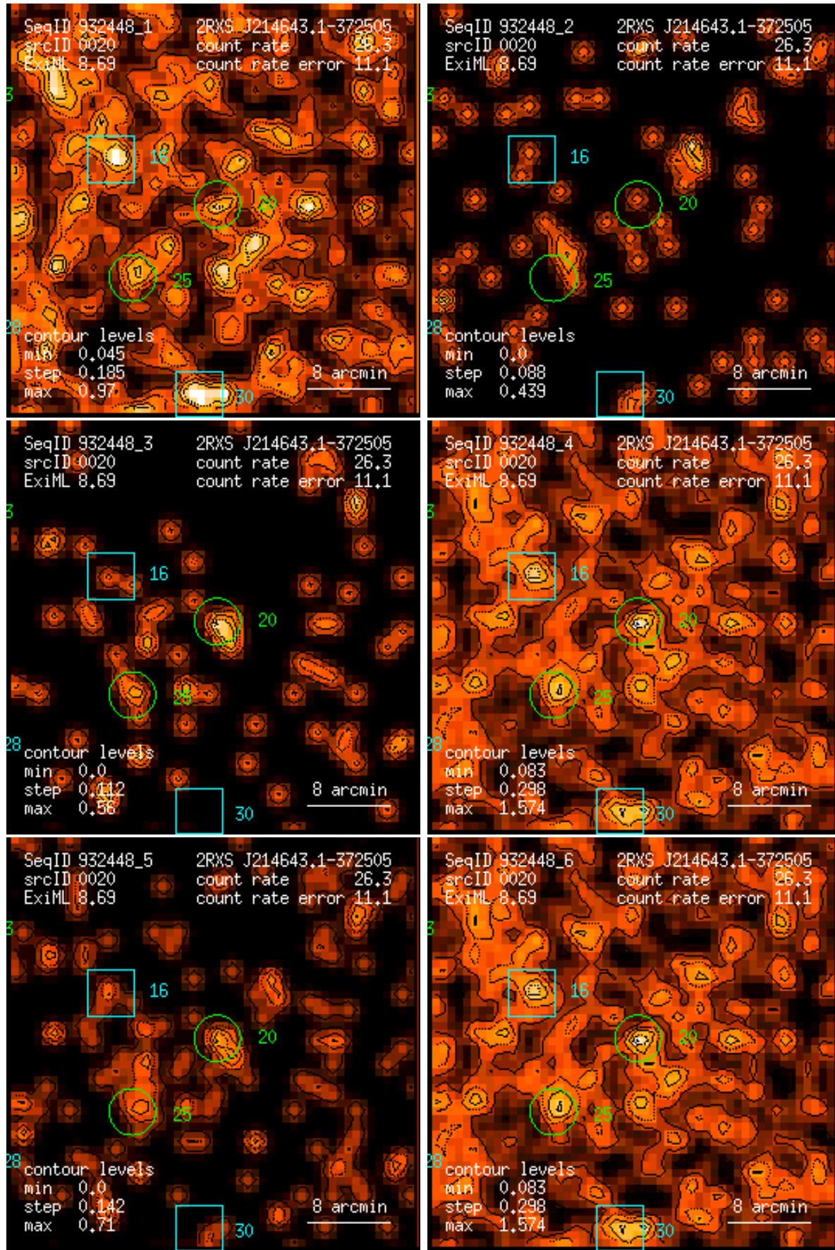
Figure 20: RASS 932448: detection 0020: band rate images, Gaussian filter: (1) PSPC channels 11 – 41, (2) 52 – 90, (3) 91 – 201, (4) 11 – 235, (5) 52 – 201, (6) 11 – 201. Broad band rates in counts/ks. Band rate contour levels in counts/ks/arcmin 2 .
