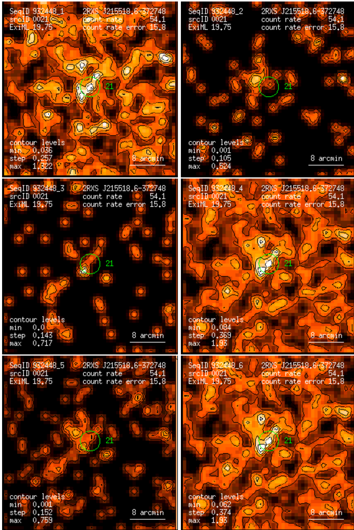
Figure 21: RASS 932448: detection 0021: band rate images, Gaussian filter: (1) PSPC channels 11 – 41, (2) 52 – 90, (3) 91 – 201, (4) 11 – 235, (5) 52 – 201, (6) 11 – 201. Broad band rates in counts/ks. Band rate contour levels in counts/ks/arcmin 2 .
