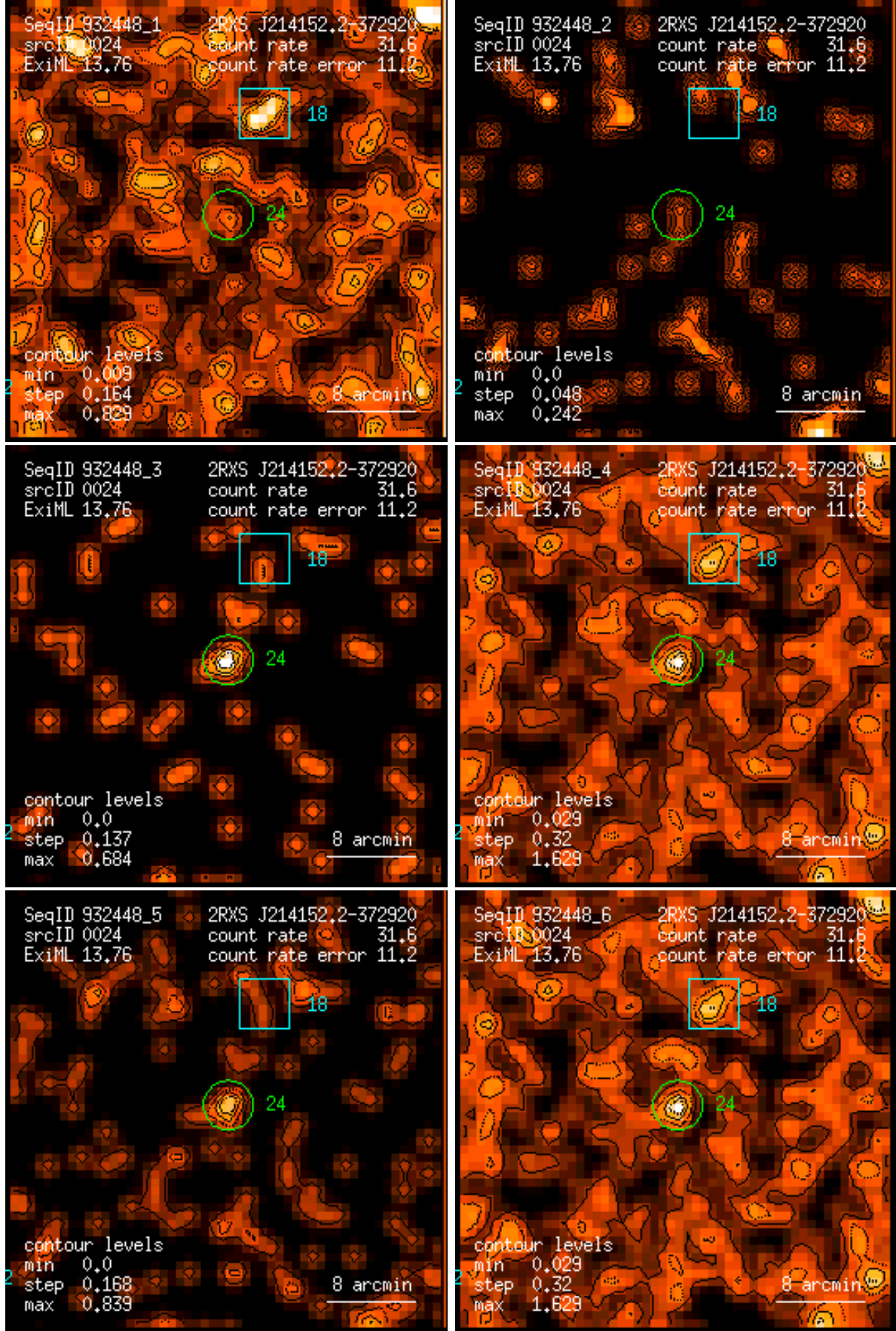
Figure 24: RASS 932448: detection 0024: band rate images, Gaussian filter: (1) PSPC channels 11 – 41, (2) 52 – 90, (3) 91 – 201, (4) 11 – 235, (5) 52 – 201, (6) 11 – 201. Broad band rates in counts/ks. Band rate contour levels in counts/ks/arcmin 2 .
