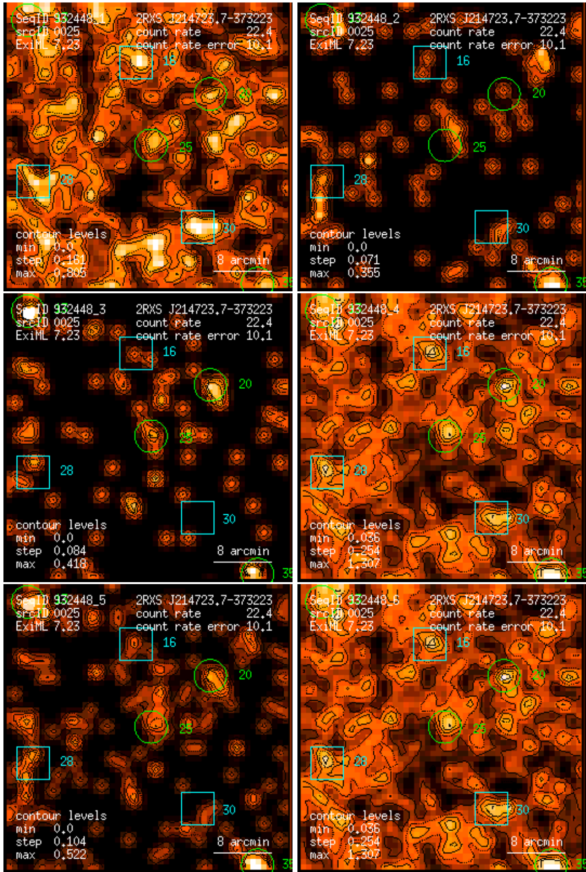
Figure 25: RASS 932448: detection 0025: band rate images, Gaussian filter: (1) PSPC channels 11 – 41, (2) 52 – 90, (3) 91 – 201, (4) 11 – 235, (5) 52 – 201, (6) 11 – 201. Broad band rates in counts/ks. Band rate contour levels in counts/ks/arcmin 2 .
