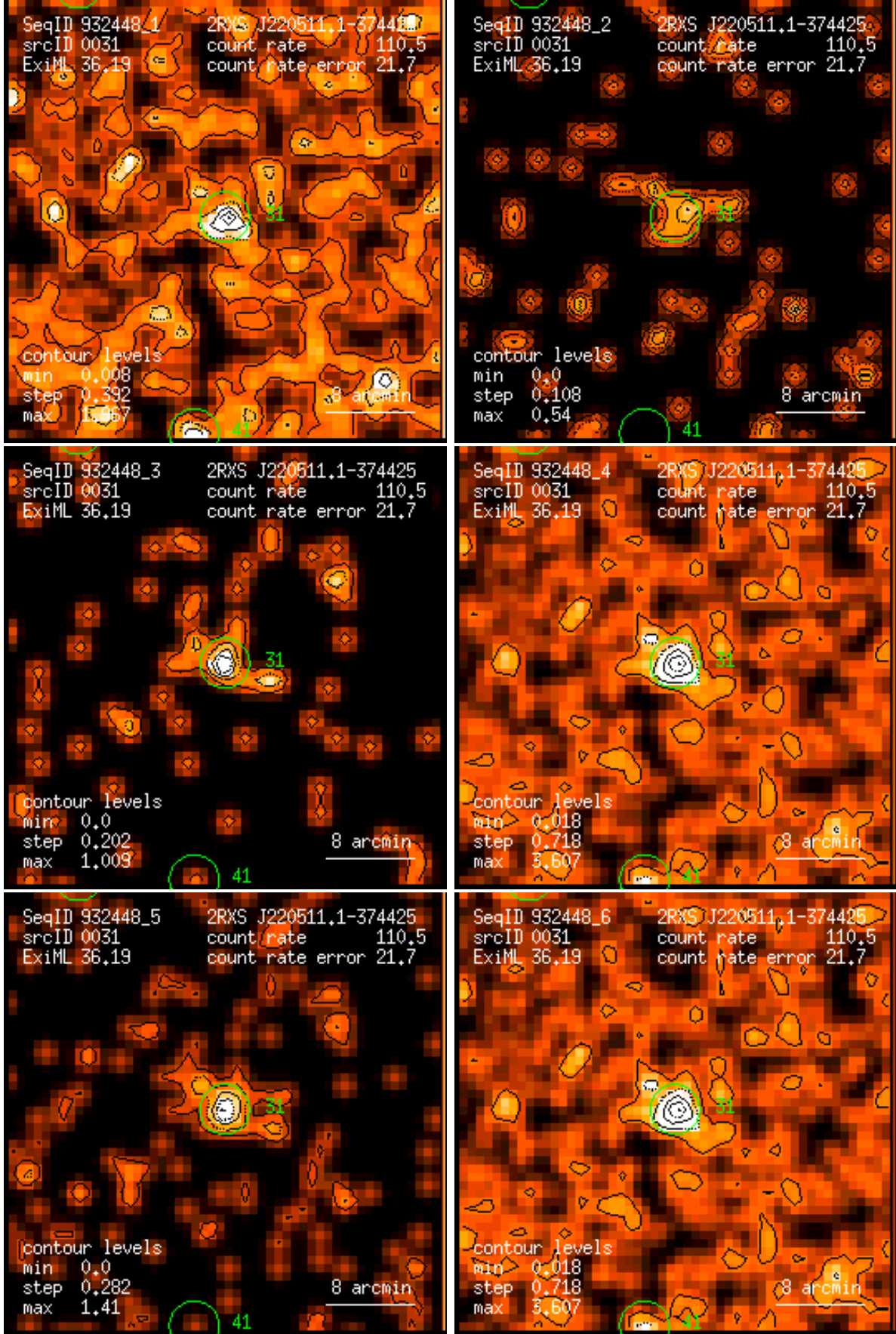
Figure 31: RASS 932448: detection 0031: band rate images, Gaussian filter: (1) PSPC channels 11 – 41, (2) 52 – 90, (3) 91 – 201, (4) 11 – 235, (5) 52 – 201, (6) 11 – 201. Broad band rates in counts/ks. Band rate contour levels in counts/ks/arcmin 2 .
