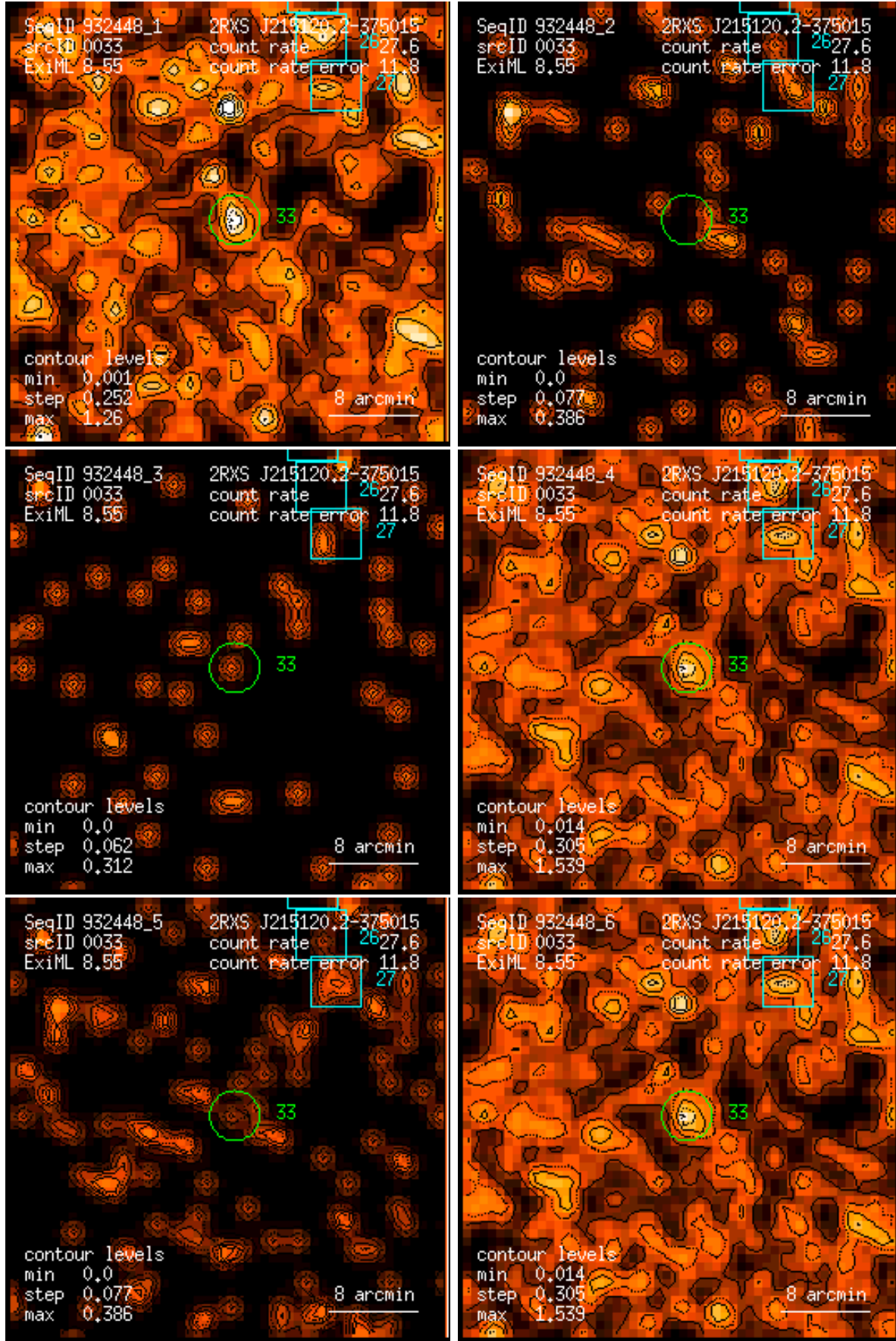
Figure 33: RASS 932448: detection 0033: band rate images, Gaussian filter: (1) PSPC channels 11 – 41, (2) 52 – 90, (3) 91 – 201, (4) 11 – 235, (5) 52 – 201, (6) 11 – 201. Broad band rates in counts/ks. Band rate contour levels in counts/ks/arcmin 2 .
