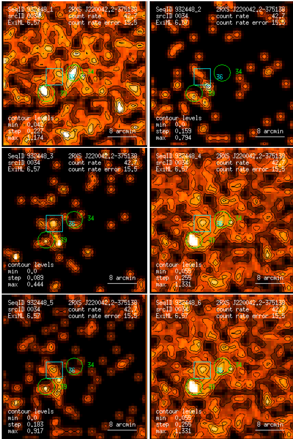
Figure 34: RASS 932448: detection 0034: band rate images, Gaussian filter: (1) PSPC channels 11 – 41, (2) 52 – 90, (3) 91 – 201, (4) 11 – 235, (5) 52 – 201, (6) 11 – 201. Broad band rates in counts/ks. Band rate contour levels in counts/ks/arcmin 2 .
