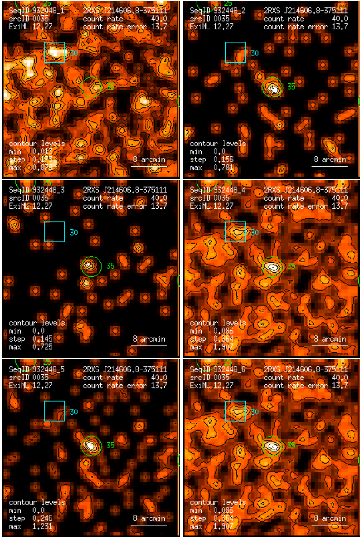
Figure 35: RASS 932448: detection 0035: band rate images, Gaussian filter: (1) PSPC channels 11 – 41, (2) 52 – 90, (3) 91 – 201, (4) 11 – 235, (5) 52 – 201, (6) 11 – 201. Broad band rates in counts/ks. Band rate contour levels in counts/ks/arcmin 2 .
