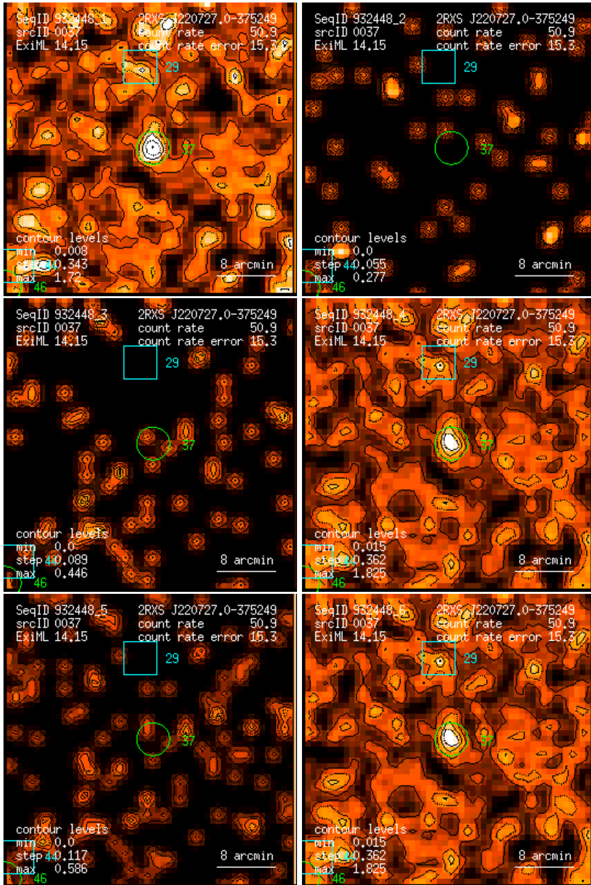
Figure 37: RASS 932448: detection 0037: band rate images, Gaussian filter: (1) PSPC channels 11 – 41, (2) 52 – 90, (3) 91 – 201, (4) 11 – 235, (5) 52 – 201, (6) 11 – 201. Broad band rates in counts/ks. Band rate contour levels in counts/ks/arcmin 2 .
