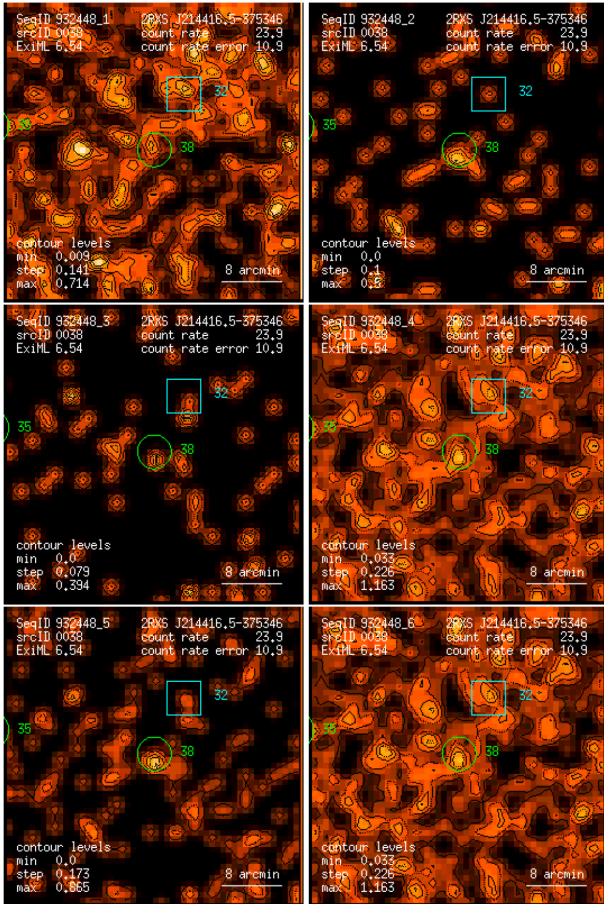
Figure 38: RASS 932448: detection 0038: band rate images, Gaussian filter: (1) PSPC channels 11 – 41, (2) 52 – 90, (3) 91 – 201, (4) 11 – 235, (5) 52 – 201, (6) 11 – 201. Broad band rates in counts/ks. Band rate contour levels in counts/ks/arcmin 2 .
