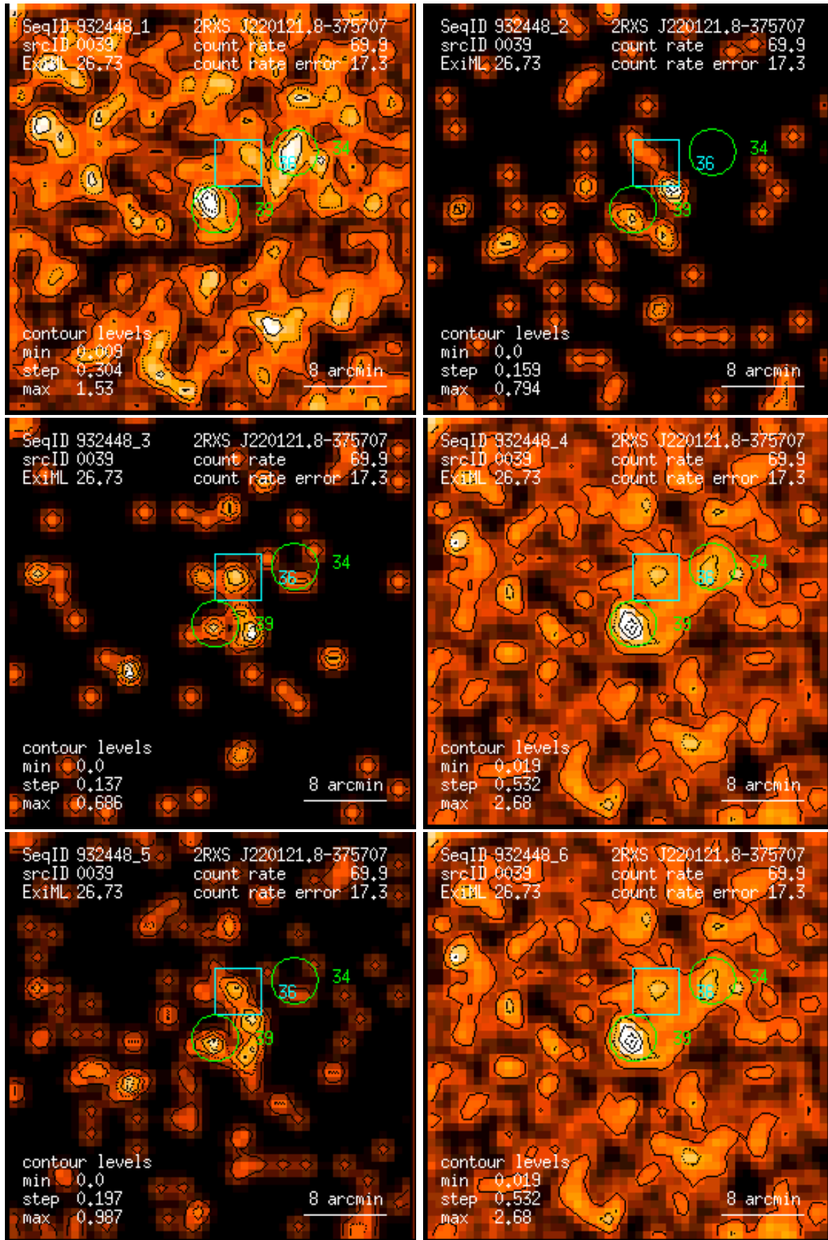
Figure 39: RASS 932448: detection 0039: band rate images, Gaussian filter: (1) PSPC channels 11 – 41, (2) 52 – 90, (3) 91 – 201, (4) 11 – 235, (5) 52 – 201, (6) 11 – 201. Broad band rates in counts/ks. Band rate contour levels in counts/ks/arcmin 2 .
