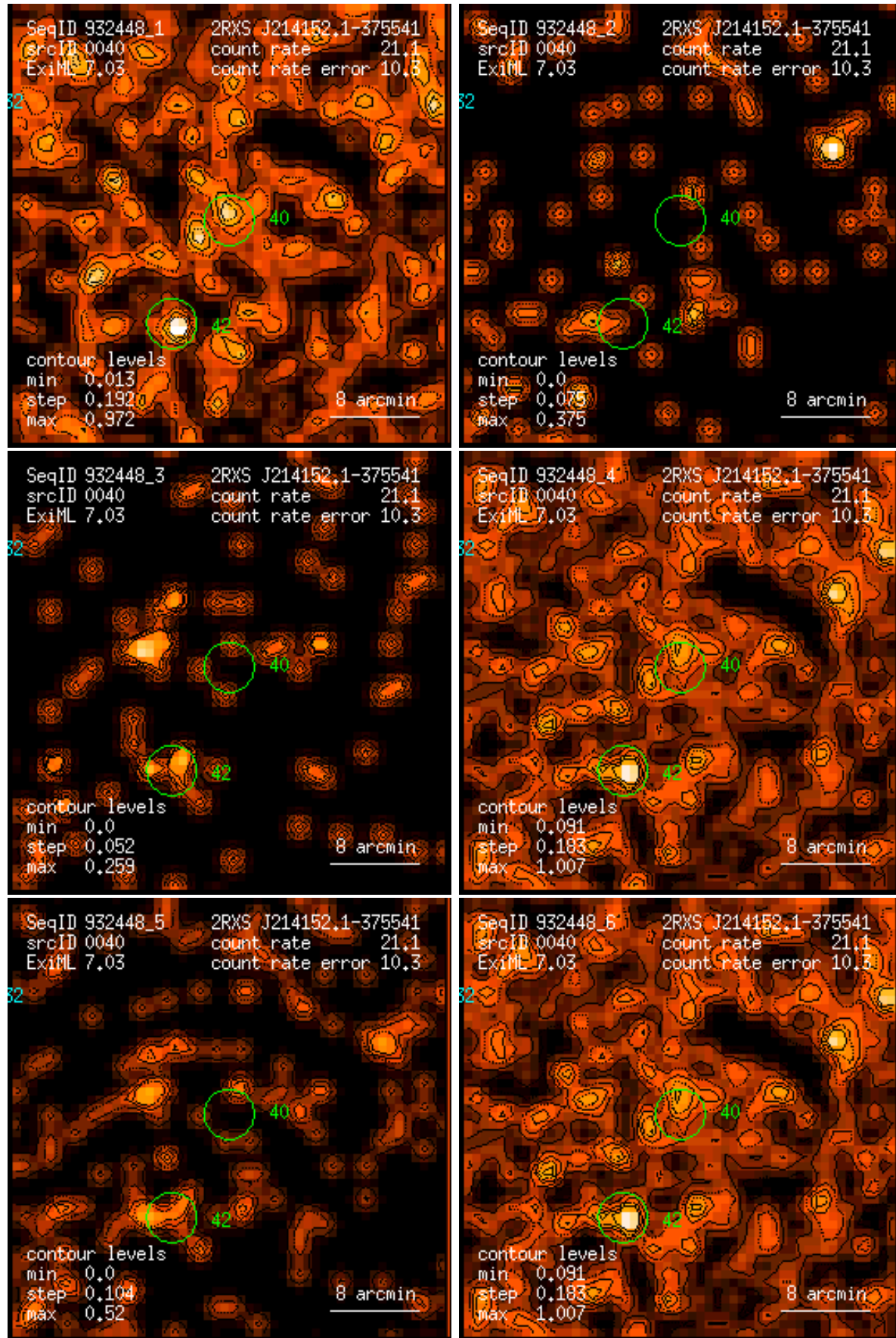
Figure 40: RASS 932448: detection 0040: band rate images, Gaussian filter: (1) PSPC channels 11 – 41, (2) 52 – 90, (3) 91 – 201, (4) 11 – 235, (5) 52 – 201, (6) 11 – 201. Broad band rates in counts/ks. Band rate contour levels in counts/ks/arcmin 2 .
