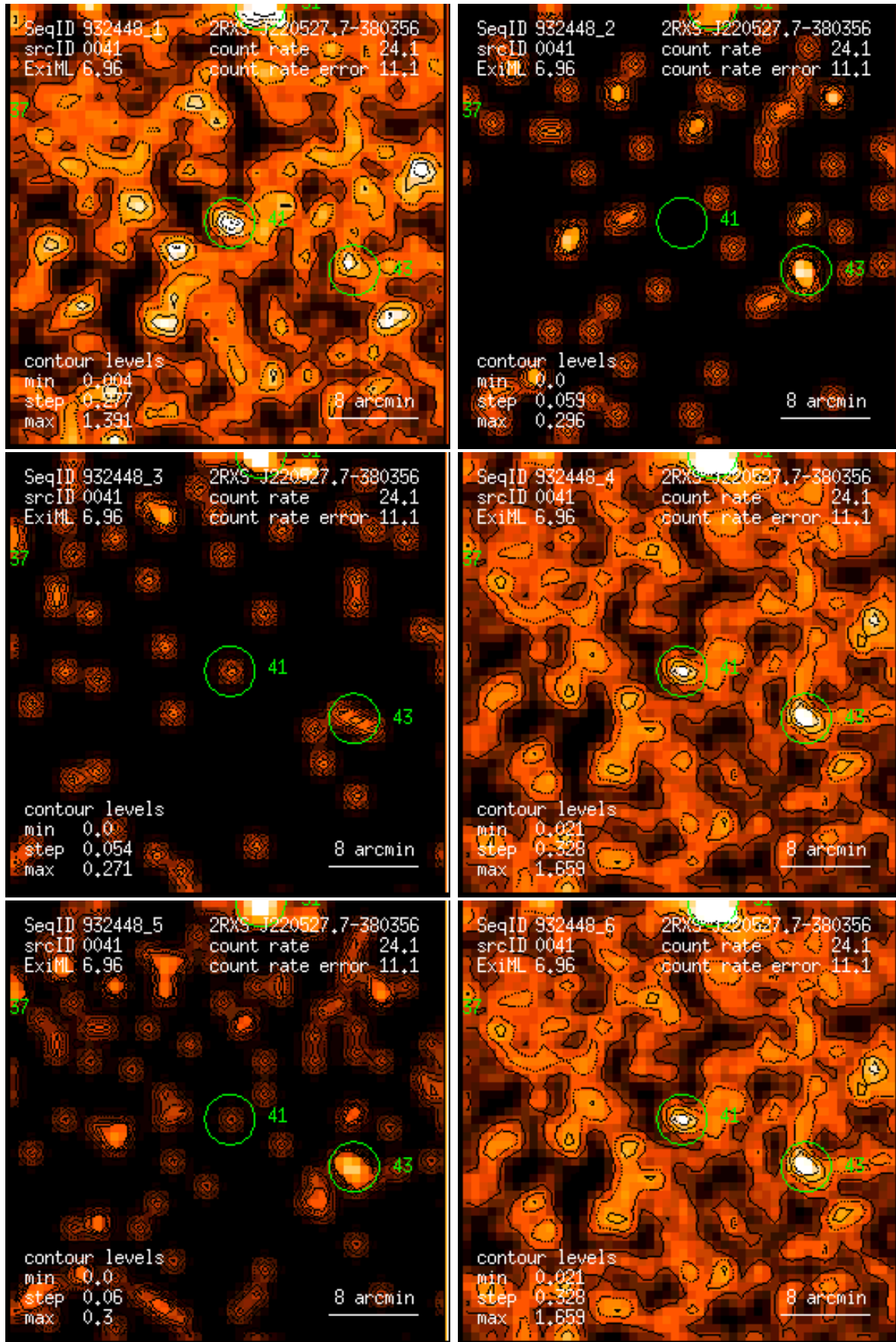
Figure 41: RASS 932448: detection 0041: band rate images, Gaussian filter: (1) PS7 channels 11 – 41, (2) PS8 52 – 90, (3) PS9 91 – 201, (4) PS10 11 – 235, (5) PS11 52 – 201, (6) PS12 11 – 201. Broad band rates in counts/ks. Band rate contour levels in counts/ks/arcmin 2 .
