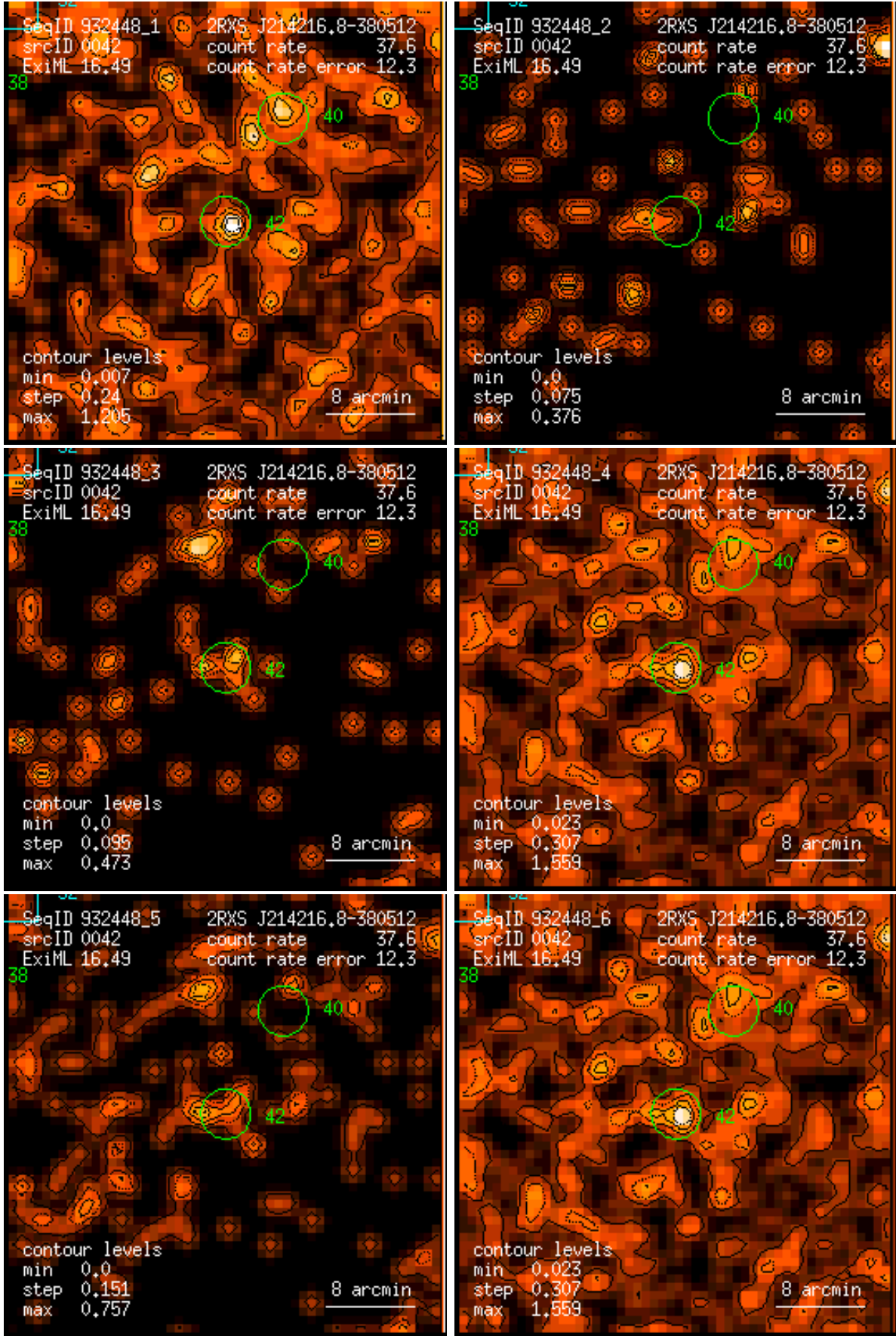
Figure 42: RASS 932448: detection 0042: band rate images, Gaussian filter: (1) PSPC channels 11 – 41, (2) 52 – 90, (3) 91 – 201, (4) 11 – 235, (5) 52 – 201, (6) 11 – 201. Broad band rates in counts/ks. Band rate contour levels in counts/ks/arcmin 2 .
