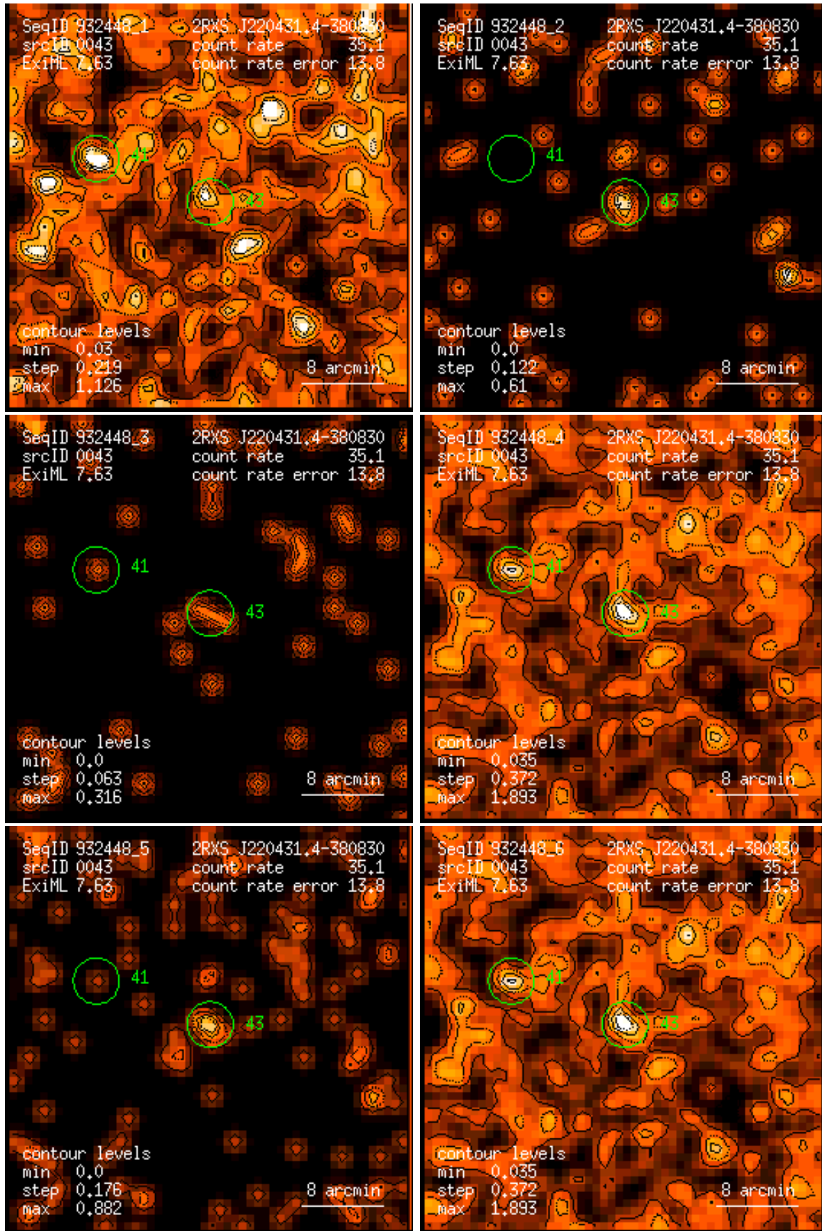
Figure 43: RASS 932448: detection 0043: band rate images, Gaussian filter: (1) PSPC channels 11 – 41, (2) 52 – 90, (3) 91 – 201, (4) 11 – 235, (5) 52 – 201, (6) 11 – 201. Broad band rates in counts/ks. Band rate contour levels in counts/ks/arcmin 2 .
