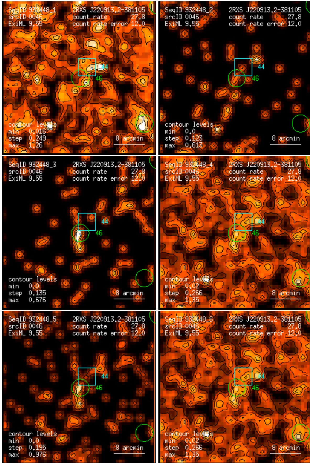
Figure 46: RASS 932448: detection 0046: band rate images, Gaussian filter: (1) PSPC channels 11 – 41, (2) 52 – 90, (3) 91 – 201, (4) 11 – 235, (5) 52 – 201, (6) 11 – 201. Broad band rates in counts/ks. Band rate contour levels in counts/ks/arcmin 2 .
