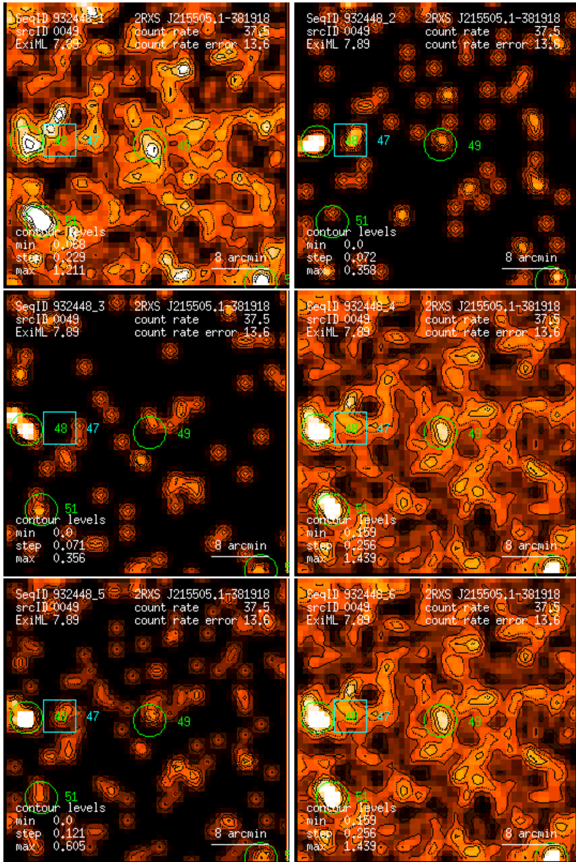
Figure 49: RASS 932448: detection 0049: band rate images, Gaussian filter: (1) PSPC channels 11 – 41, (2) 52 – 90, (3) 91 – 201, (4) 11 – 235, (5) 52 – 201, (6) 11 – 201. Broad band rates in counts/ks. Band rate contour levels in counts/ks/arcmin 2 .
