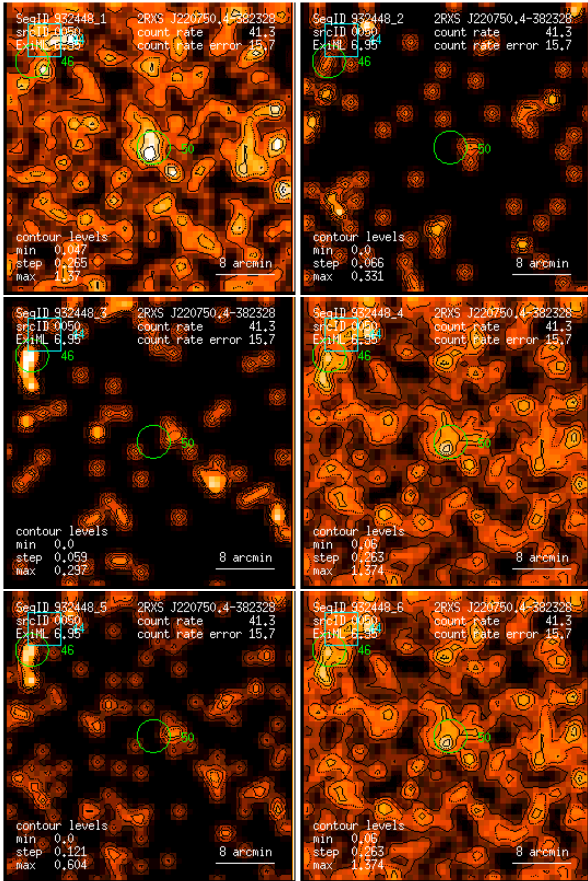
Figure 50: RASS 932448: detection 0050: band rate images, Gaussian filter: (1) PSPC channels 11 – 41, (2) 52 – 90, (3) 91 – 201, (4) 11 – 235, (5) 52 – 201, (6) 11 – 201. Broad band rates in counts/ks. Band rate contour levels in counts/ks/arcmin 2 .
