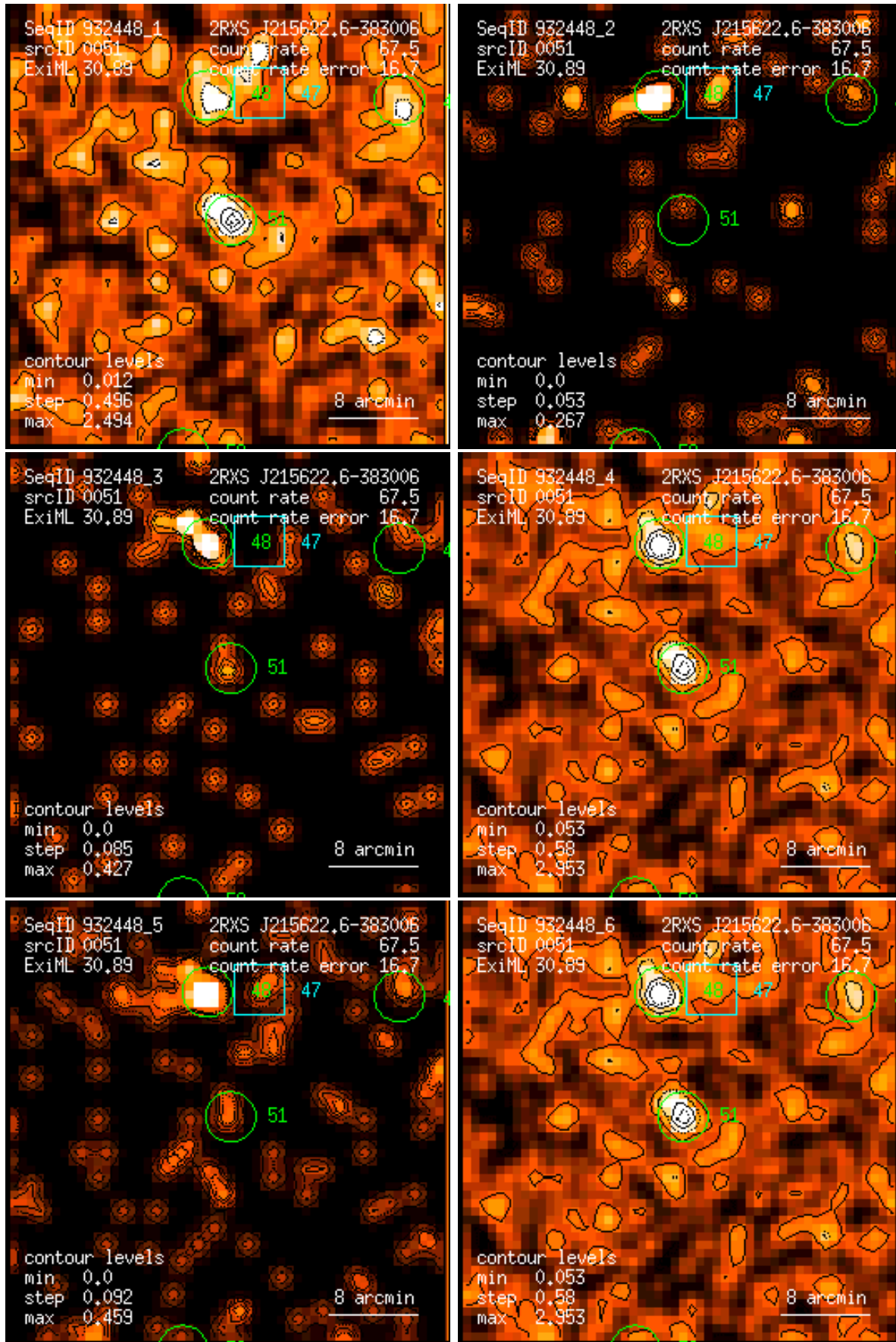
Figure 51: RASS 932448: detection 0051: band rate images, Gaussian filter: (1) PSPC channels 11 – 41, (2) 52 – 90, (3) 91 – 201, (4) 11 – 235, (5) 52 – 201, (6) 11 – 201. Broad band rates in counts/ks. Band rate contour levels in counts/ks/arcmin 2 .
