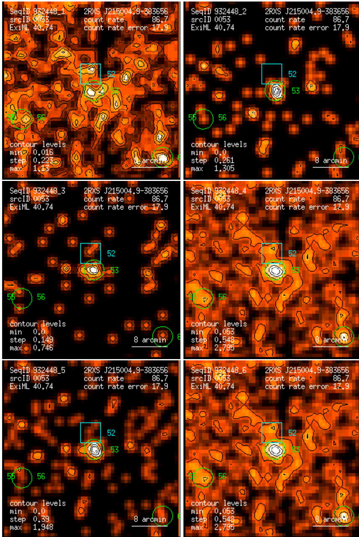
Figure 53: RASS 932448: detection 0053: band rate images, Gaussian filter: (1) PSPC channels 11 – 41, (2) 52 – 90, (3) 91 – 201, (4) 11 – 235, (5) 52 – 201, (6) 11 – 201. Broad band rates in counts/ks. Band rate contour levels in counts/ks/arcmin 2 .
