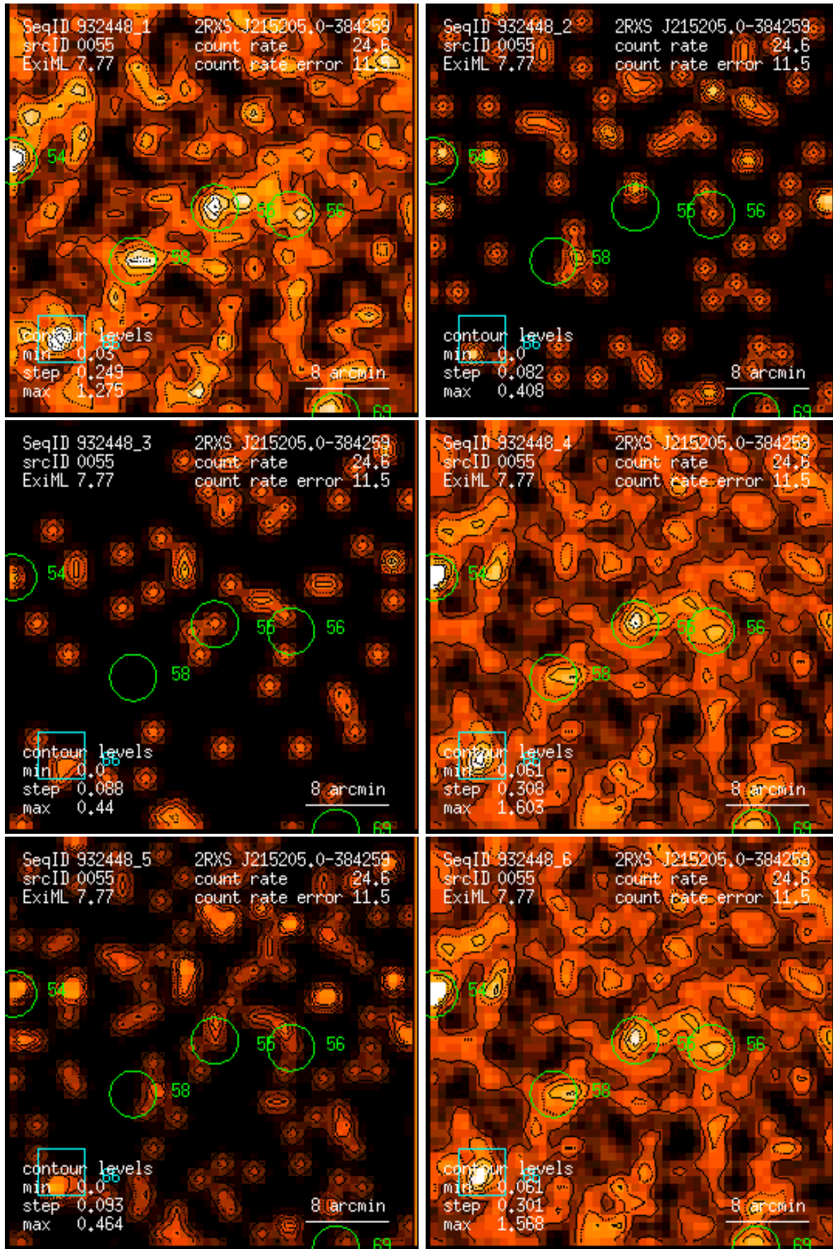
Figure 55: RASS 932448: detection 0055: band rate images, Gaussian filter: (1) PSPC channels 11 – 41, (2) 52 – 90, (3) 91 – 201, (4) 11 – 235, (5) 52 – 201, (6) 11 – 201. Broad band rates in counts/ks. Band rate contour levels in counts/ks/arcmin 2 .
