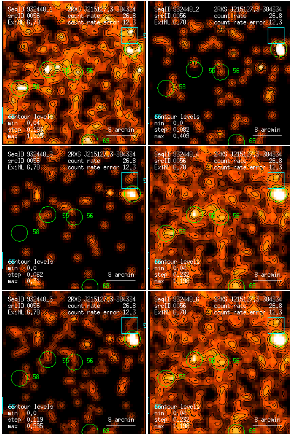
Figure 56: RASS 932448: detection 0056: band rate images, Gaussian filter: (1) PSPC channels 11 – 41, (2) 52 – 90, (3) 91 – 201, (4) 11 – 235, (5) 52 – 201, (6) 11 – 201. Broad band rates in counts/ks. Band rate contour levels in counts/ks/arcmin 2 .
