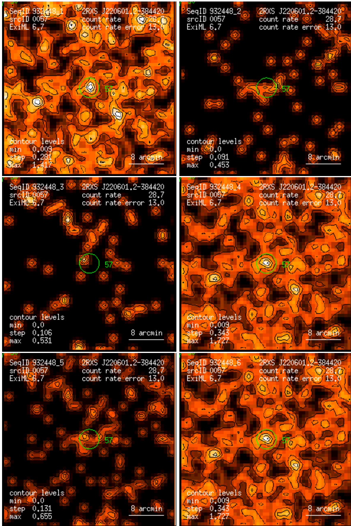
Figure 57: RASS 932448: detection 0057: band rate images, Gaussian filter: (1) PSPC channels 11 – 41, (2) 52 – 90, (3) 91 – 201, (4) 11 – 235, (5) 52 – 201, (6) 11 – 201. Broad band rates in counts/ks. Band rate contour levels in counts/ks/arcmin 2 .
