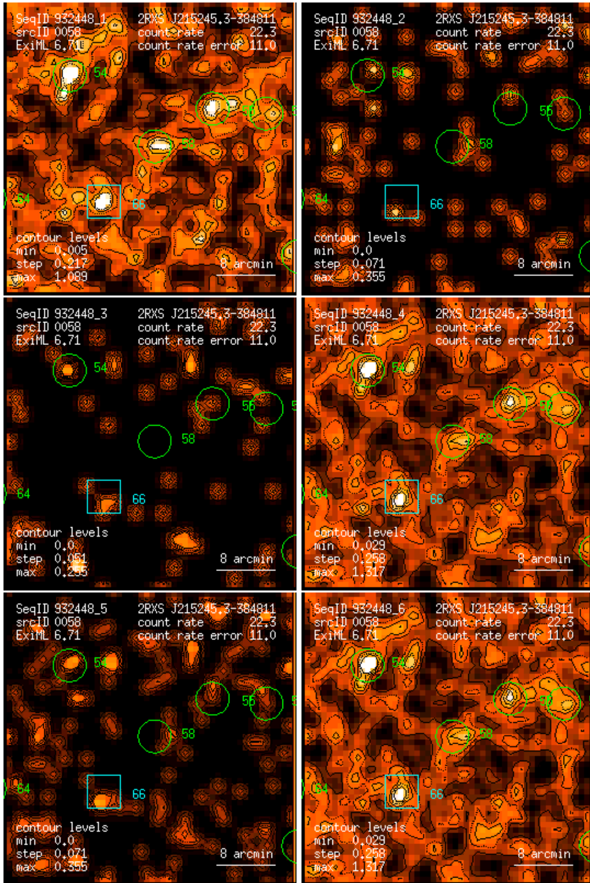
Figure 58: RASS 932448: detection 0058: band rate images, Gaussian filter: (1) PSPC channels 11 – 41, (2) 52 – 90, (3) 91 – 201, (4) 11 – 235, (5) 52 – 201, (6) 11 – 201. Broad band rates in counts/ks. Band rate contour levels in counts/ks/arcmin 2 .
