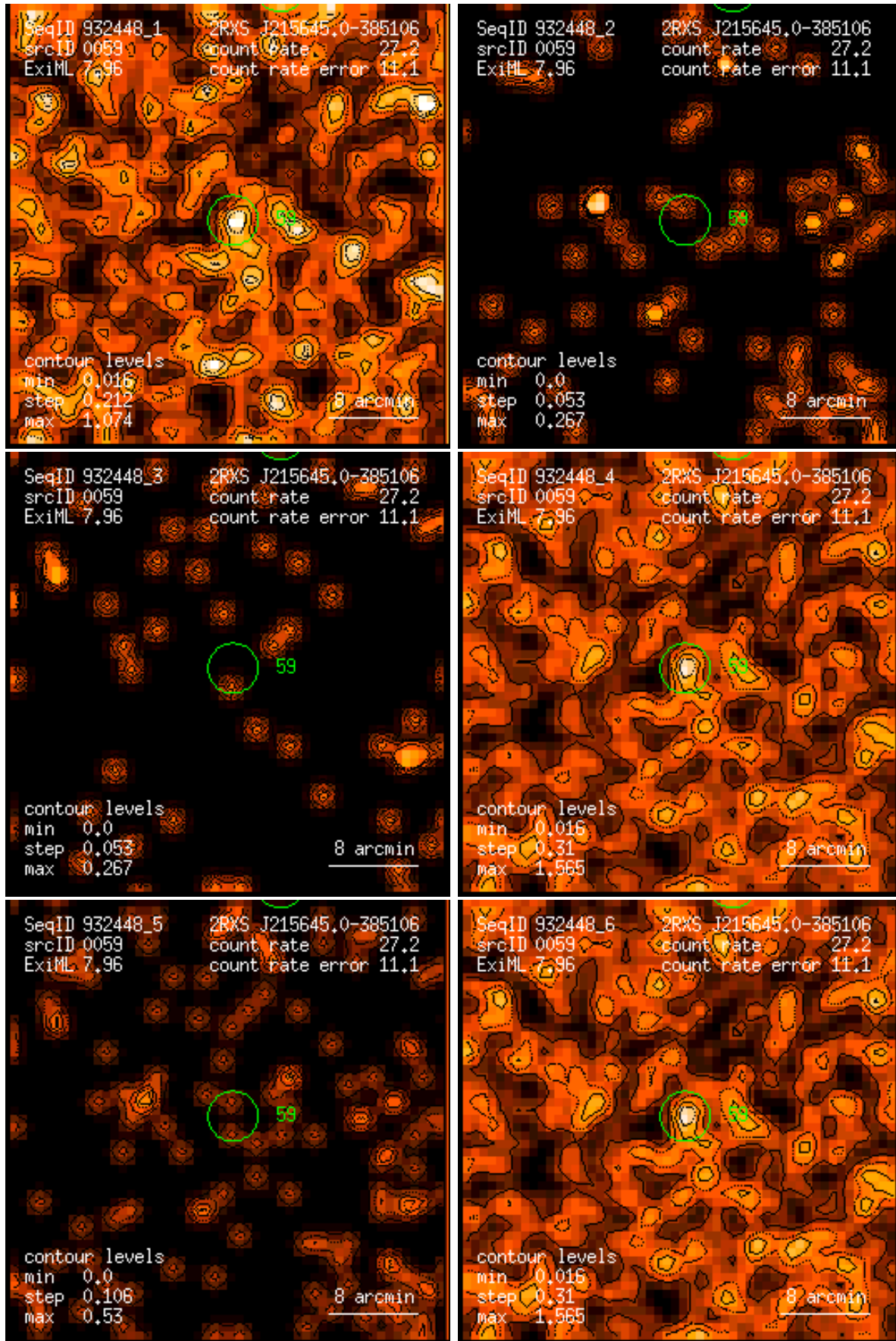
Figure 59: RASS 932448: detection 0059: band rate images, Gaussian filter: (1) PSPC channels 11 – 41, (2) 52 – 90, (3) 91 – 201, (4) 11 – 235, (5) 52 – 201, (6) 11 – 201. Broad band rates in counts/ks. Band rate contour levels in counts/ks/arcmin 2 .
