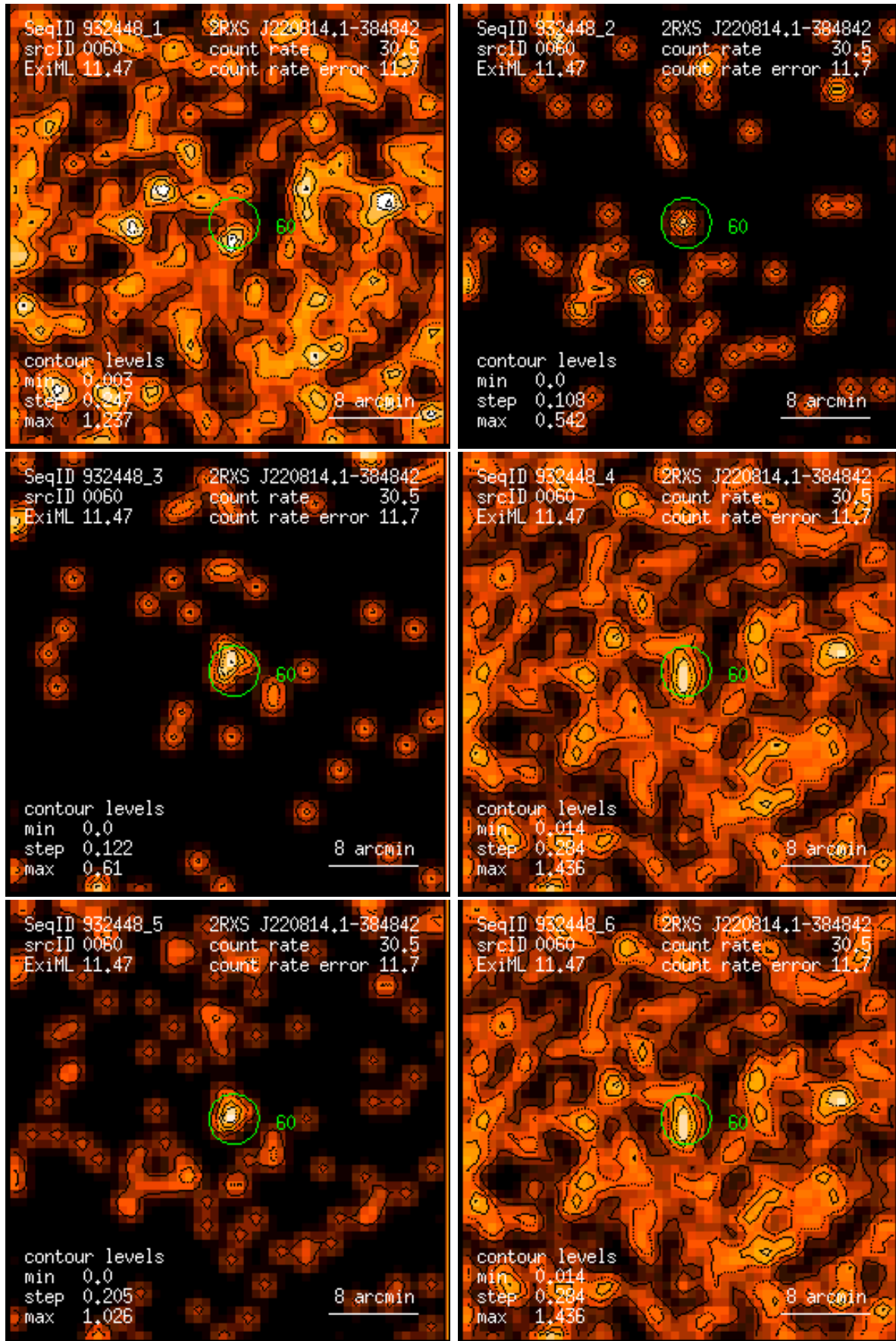
Figure 60: RASS 932448: detection 0060: band rate images, Gaussian filter: (1) PSPC channels 11 – 41, (2) 52 – 90, (3) 91 – 201, (4) 11 – 235, (5) 52 – 201, (6) 11 – 201. Broad band rates in counts/ks. Band rate contour levels in counts/ks/arcmin 2 .
