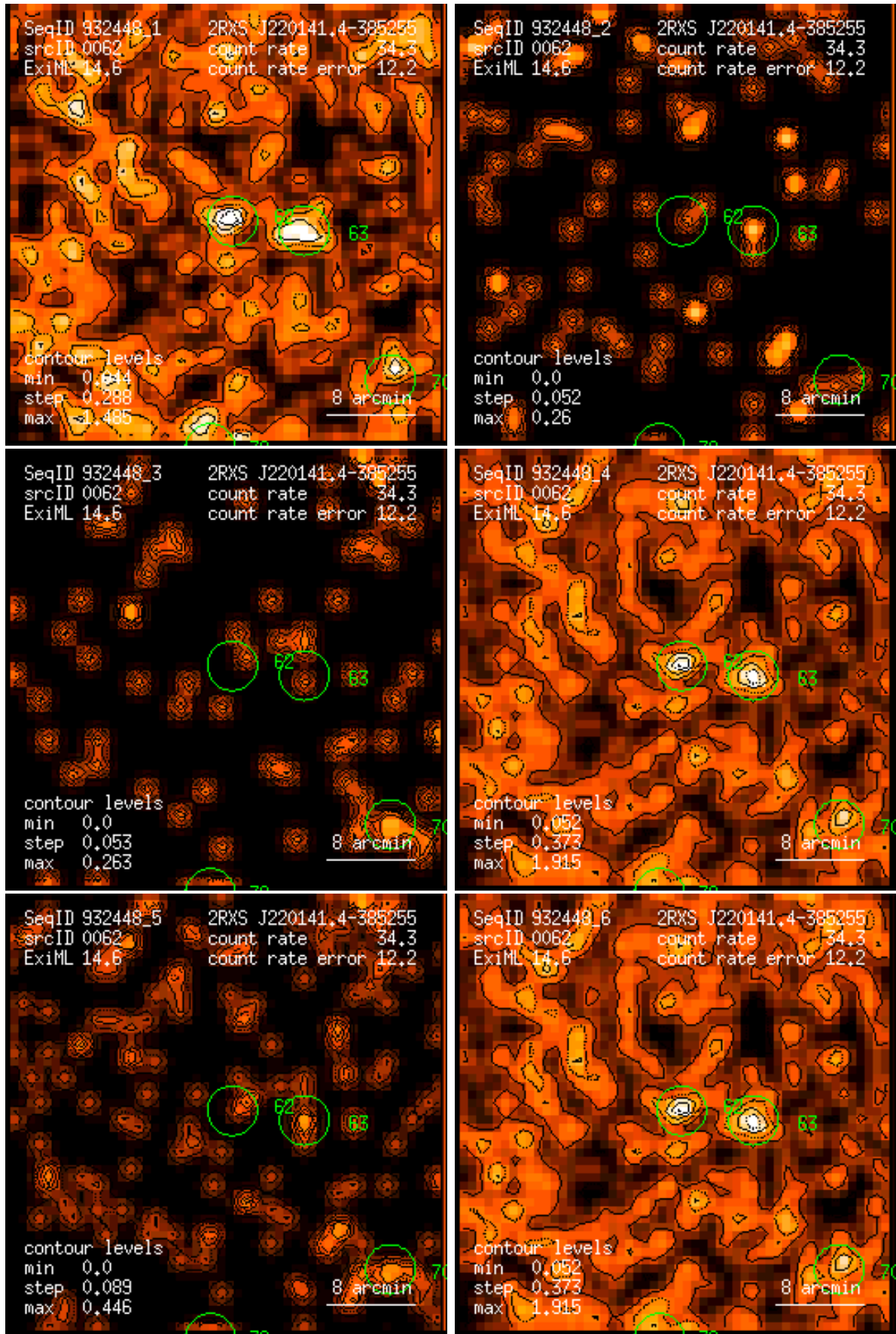
Figure 62: RASS 932448: detection 0062: band rate images, Gaussian filter: (1) PSPC channels 11 – 41, (2) 52 – 90, (3) 91 – 201, (4) 11 – 235, (5) 52 – 201, (6) 11 – 201. Broad band rates in counts/ks. Band rate contour levels in counts/ks/arcmin 2 .
