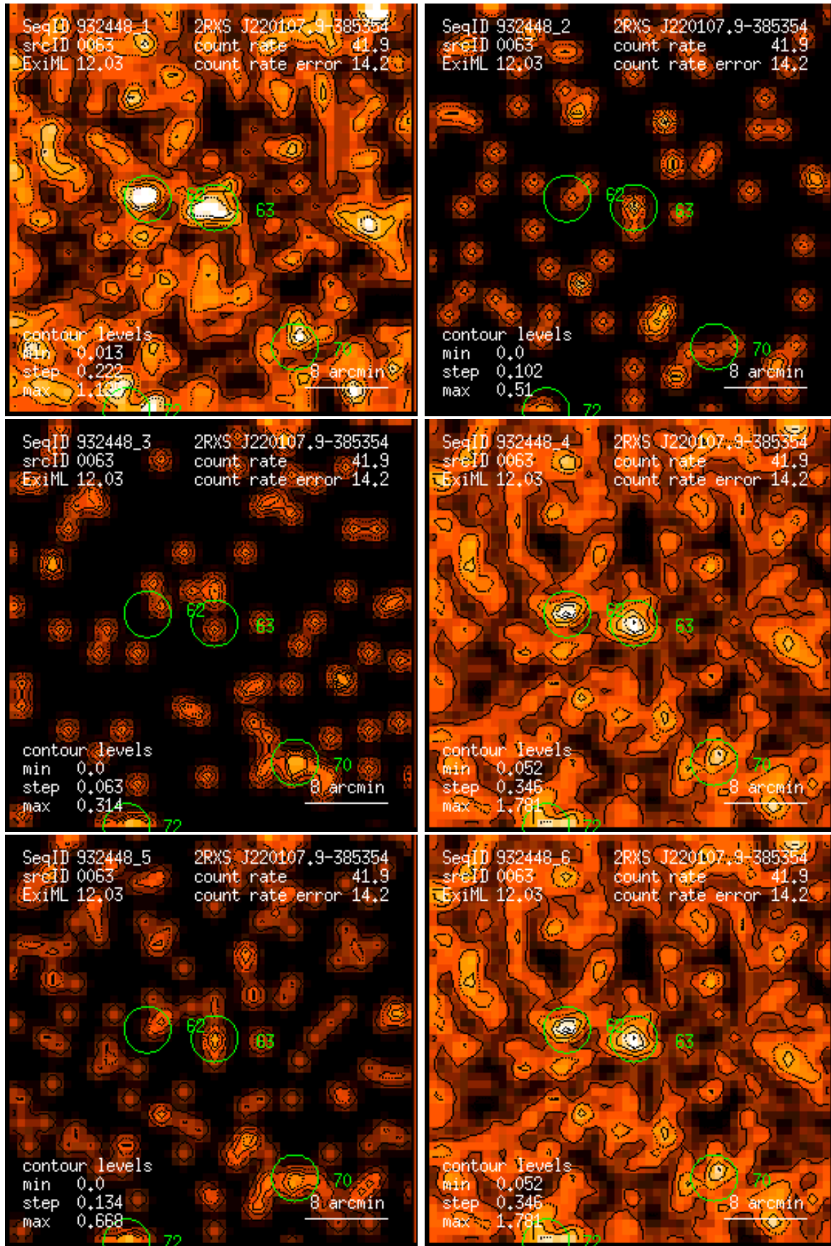
Figure 63: RASS 932448: detection 0063: band rate images, Gaussian filter: (1) PSPC channels 11 – 41, (2) 52 – 90, (3) 91 – 201, (4) 11 – 235, (5) 52 – 201, (6) 11 – 201. Broad band rates in counts/ks. Band rate contour levels in counts/ks/arcmin 2 .
