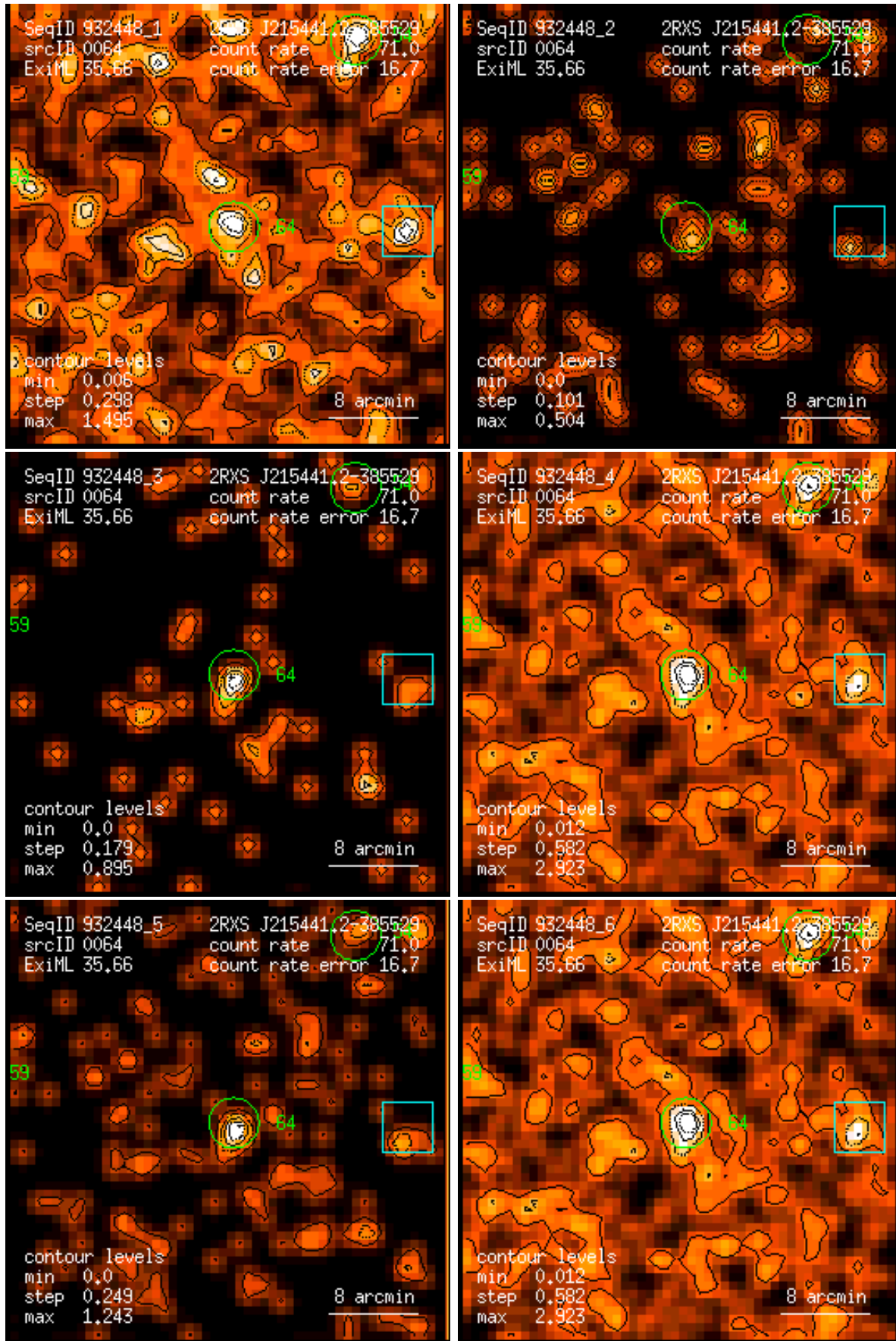
Figure 64: RASS 932448: detection 0064: band rate images, Gaussian filter: (1) PSPC channels 11 – 41, (2) 52 – 90, (3) 91 – 201, (4) 11 – 235, (5) 52 – 201, (6) 11 – 201. Broad band rates in counts/ks. Band rate contour levels in counts/ks/arcmin 2 .
