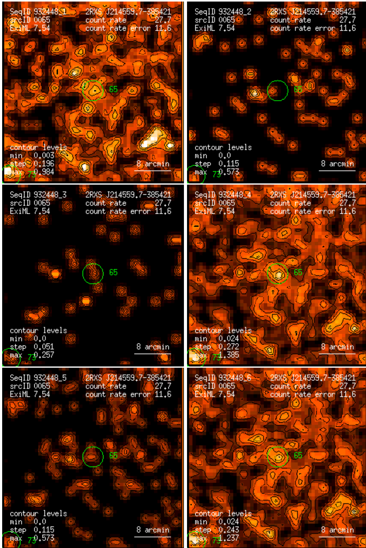
Figure 65: RASS 932448: detection 0065: band rate images, Gaussian filter: (1) PSPC channels 11 – 41, (2) 52 – 90, (3) 91 – 201, (4) 11 – 235, (5) 52 – 201, (6) 11 – 201. Broad band rates in counts/ks. Band rate contour levels in counts/ks/arcmin 2 .
