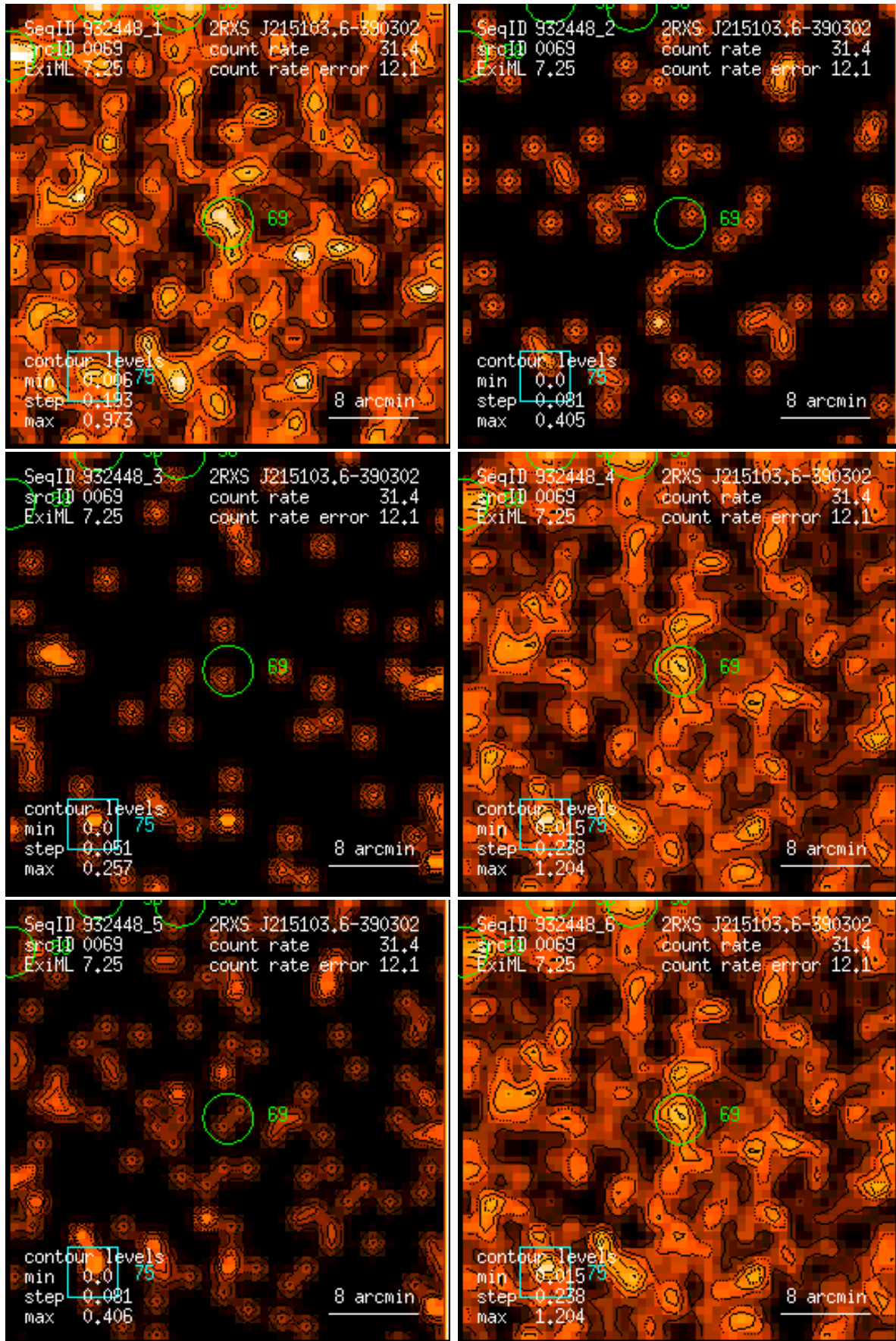
Figure 69: RASS 932448: detection 0069: band rate images, Gaussian filter: (1) PSPC channels 11 – 41, (2) 52 – 90, (3) 91 – 201, (4) 11 – 235, (5) 52 – 201, (6) 11 – 201. Broad band rates in counts/ks. Band rate contour levels in counts/ks/arcmin 2 .
