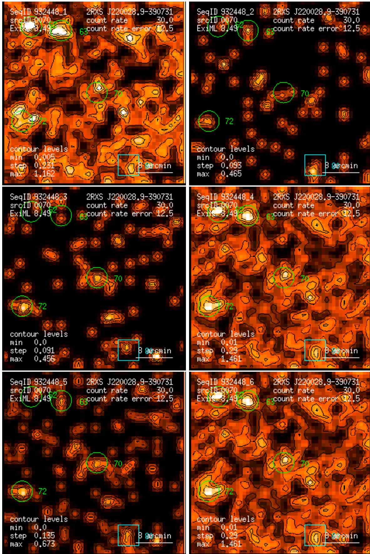
Figure 70: RASS 932448: detection 0070: band rate images, Gaussian filter: (1) PSPC channels 11 – 41, (2) 52 – 90, (3) 91 – 201, (4) 11 – 235, (5) 52 – 201, (6) 11 – 201. Broad band rates in counts/ks. Band rate contour levels in counts/ks/arcmin 2 .
