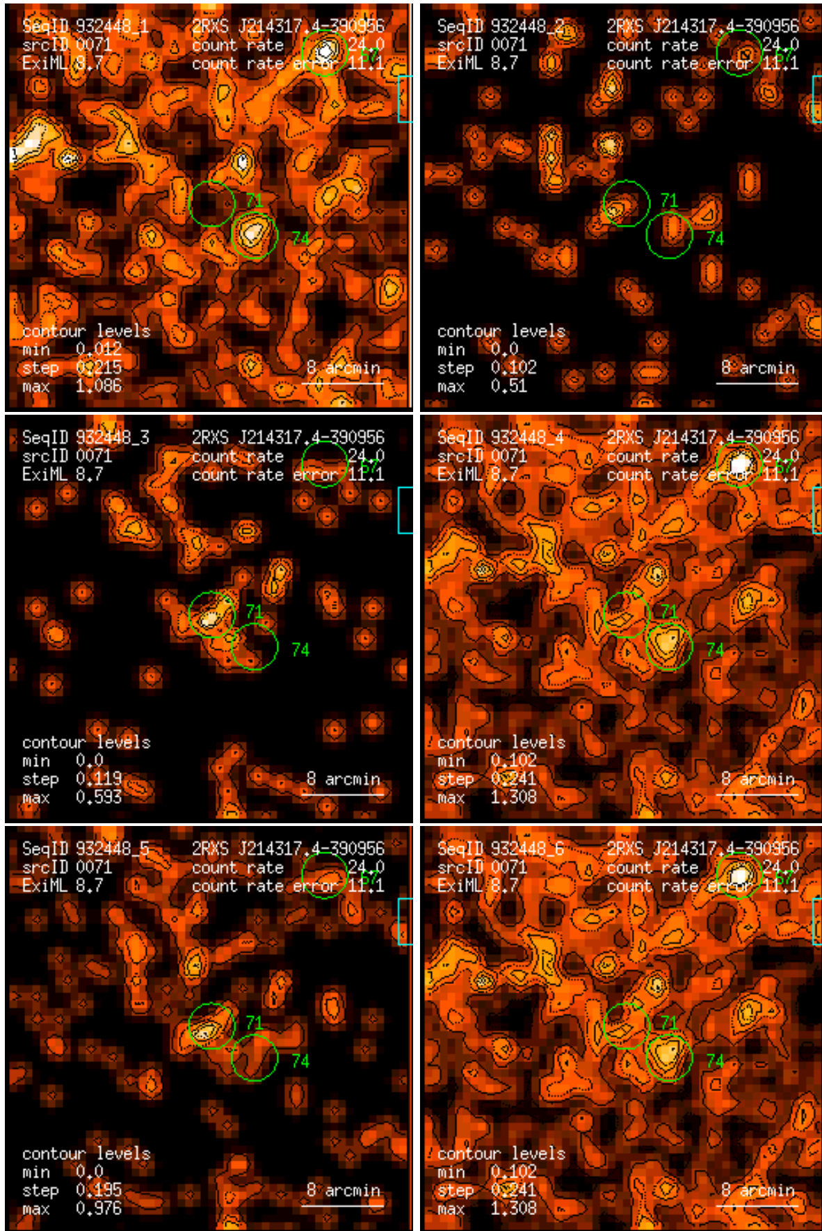
Figure 71: RASS 932448: detection 0071: band rate images, Gaussian filter: (1) PSPC channels 11 – 41, (2) 52 – 90, (3) 91 – 201, (4) 11 – 235, (5) 52 – 201, (6) 11 – 201. Broad band rates in counts/ks. Band rate contour levels in counts/ks/arcmin 2 .
