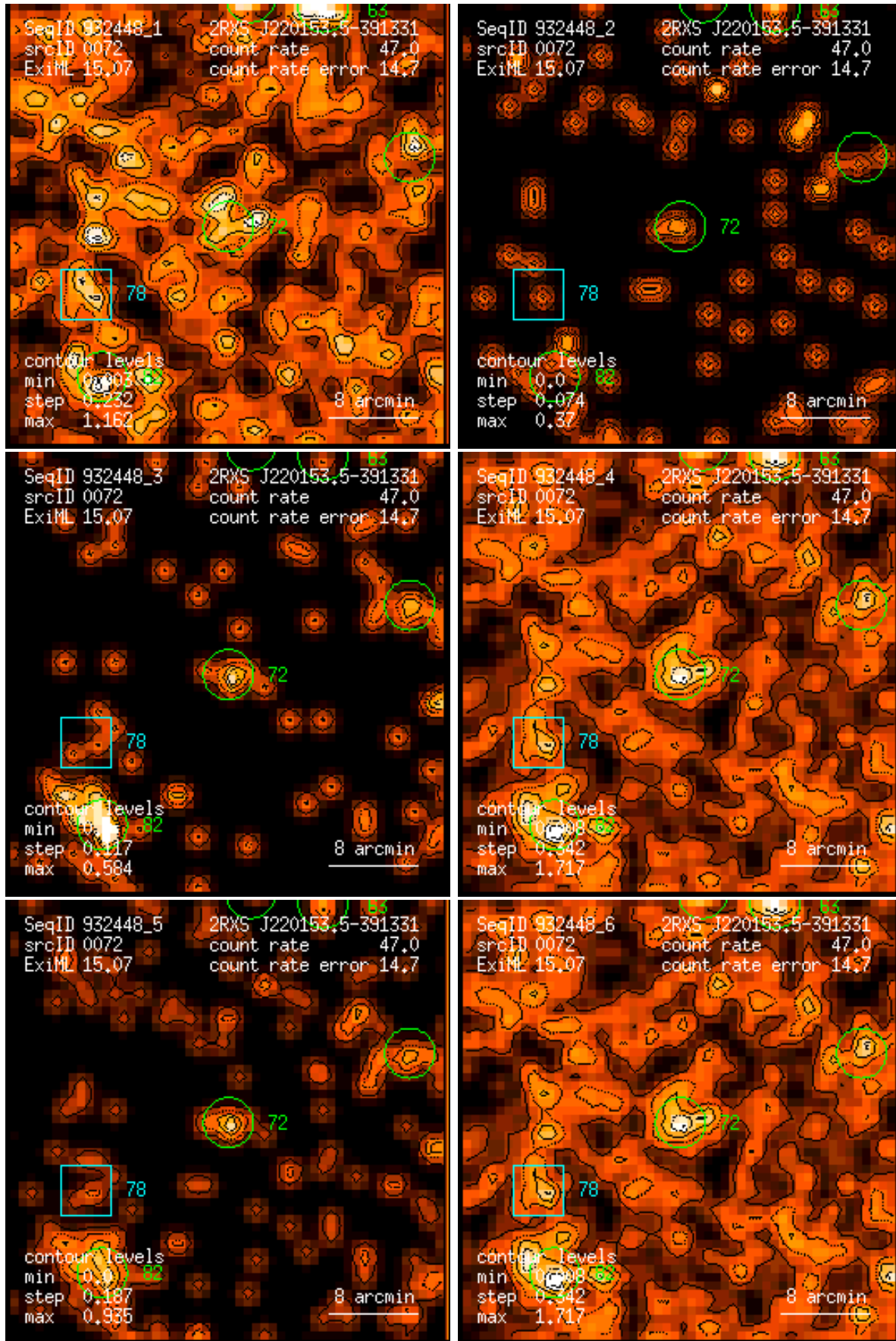
Figure 72: RASS 932448: detection 0072: band rate images, Gaussian filter: (1) PSPC channels 11 – 41, (2) 52 – 90, (3) 91 – 201, (4) 11 – 235, (5) 52 – 201, (6) 11 – 201. Broad band rates in counts/ks. Band rate contour levels in counts/ks/arcmin 2 .
