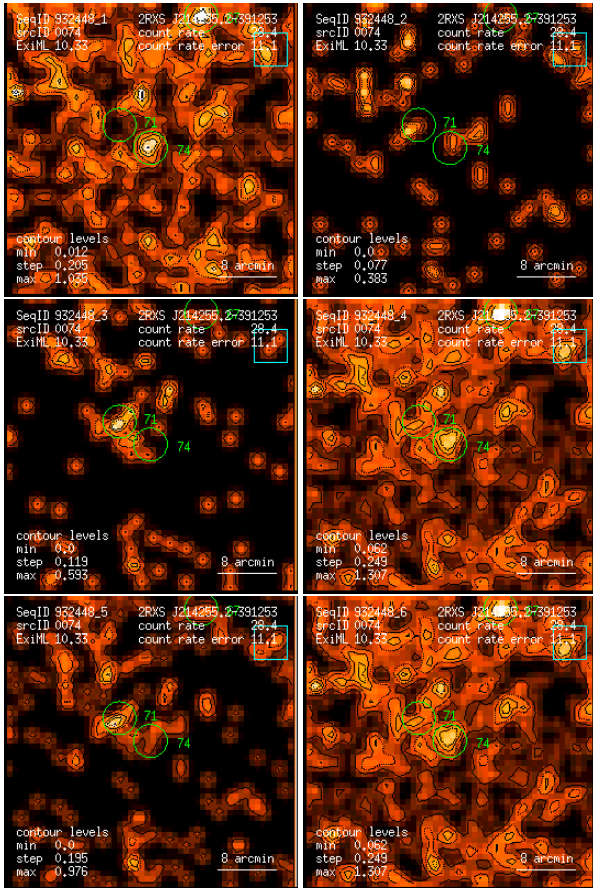
Figure 74: RASS 932448: detection 0074: band rate images, Gaussian filter: (1) PSPC channels 11 – 41, (2) 52 – 90, (3) 91 – 201, (4) 11 – 235, (5) 52 – 201, (6) 11 – 201. Broad band rates in counts/ks. Band rate contour levels in counts/ks/arcmin 2 .
