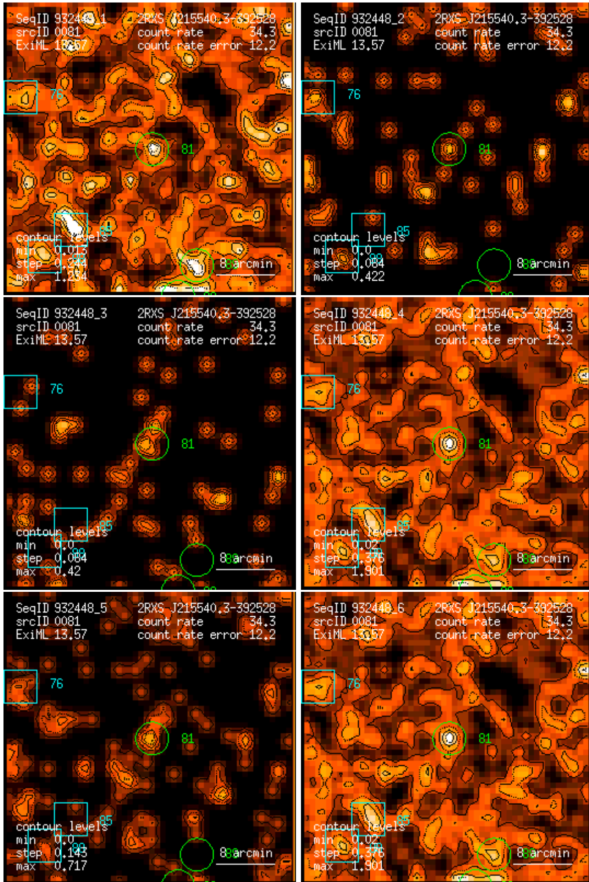
Figure 81: RASS 932448: detection 0081: band rate images, Gaussian filter: (1) PSPC channels 11 – 41, (2) 52 – 90, (3) 91 – 201, (4) 11 – 235, (5) 52 – 201, (6) 11 – 201. Broad band rates in counts/ks. Band rate contour levels in counts/ks/arcmin 2 .
