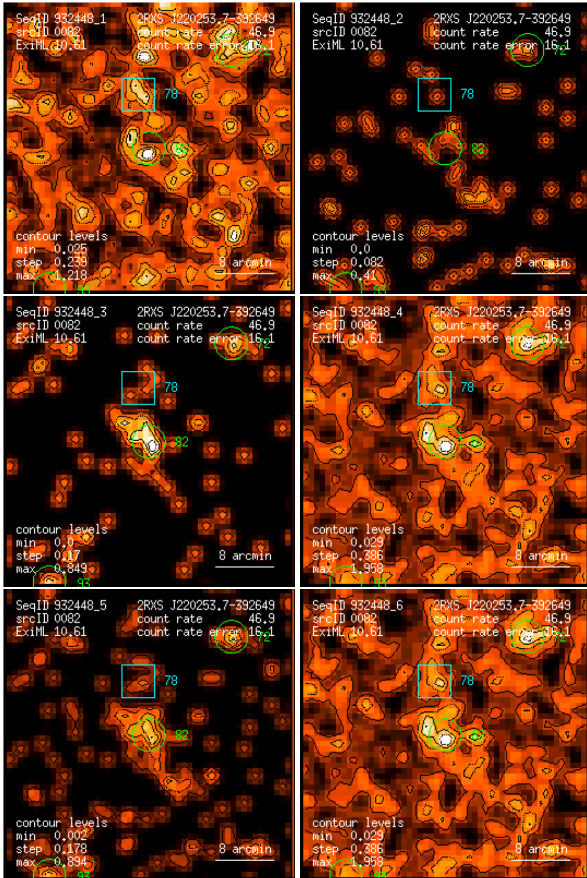
Figure 82: RASS 932448: detection 0082: band rate images, Gaussian filter: (1) PSPC channels 11 – 41, (2) 52 – 90, (3) 91 – 201, (4) 11 – 235, (5) 52 – 201, (6) 11 – 201. Broad band rates in counts/ks. Band rate contour levels in counts/ks/arcmin 2 .
