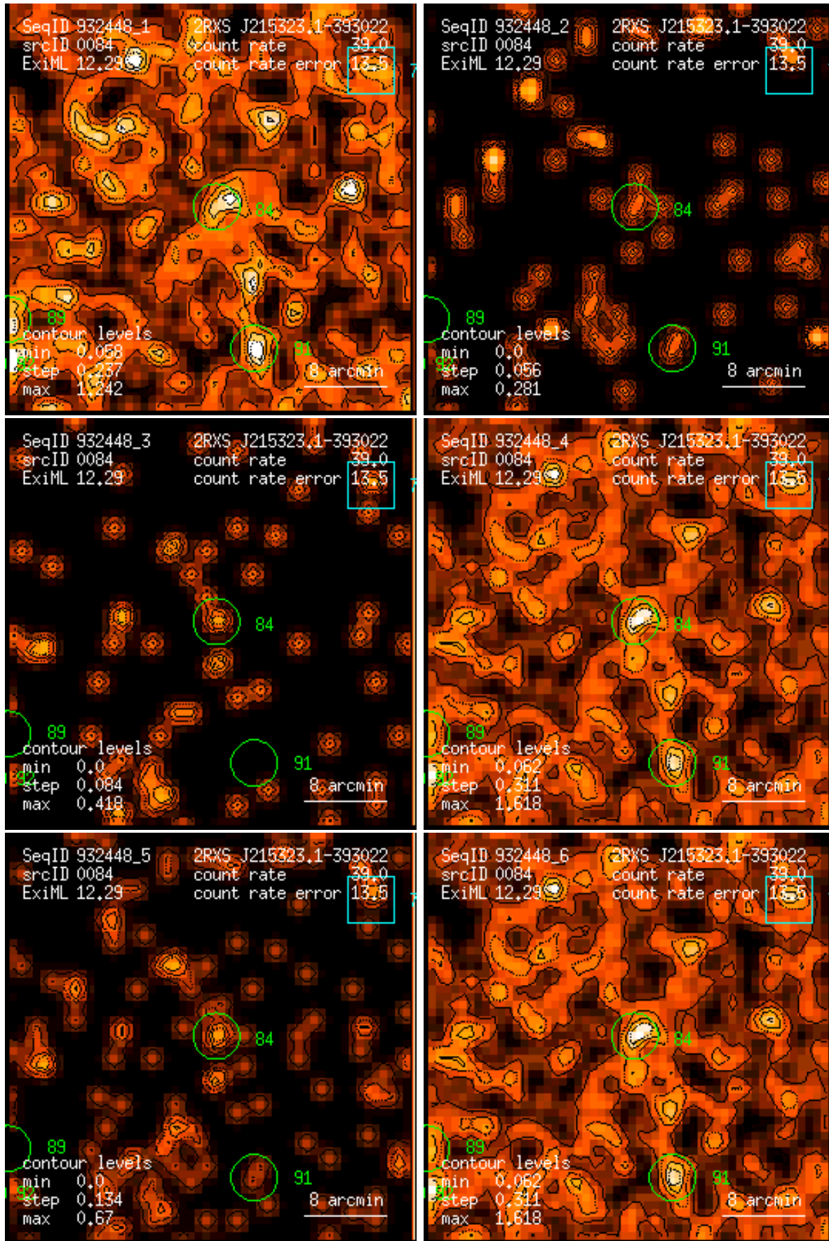
Figure 84: RASS 932448: detection 0084: band rate images, Gaussian filter: (1) PSPC channels 11 – 41, (2) 52 – 90, (3) 91 – 201, (4) 11 – 235, (5) 52 – 201, (6) 11 – 201. Broad band rates in counts/ks. Band rate contour levels in counts/ks/arcmin 2 .
