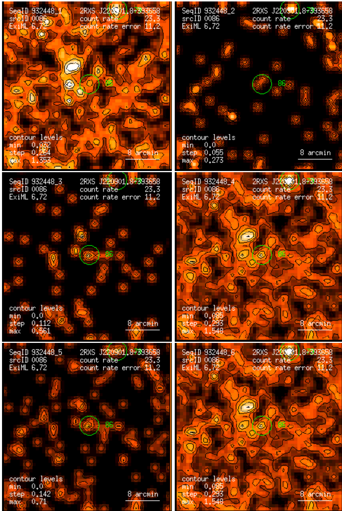
Figure 86: RASS 932448: detection 0086: band rate images, Gaussian filter: (1) PSPC channels 11 – 41, (2) 52 – 90, (3) 91 – 201, (4) 11 – 235, (5) 52 – 201, (6) 11 – 201. Broad band rates in counts/ks. Band rate contour levels in counts/ks/arcmin 2 .
