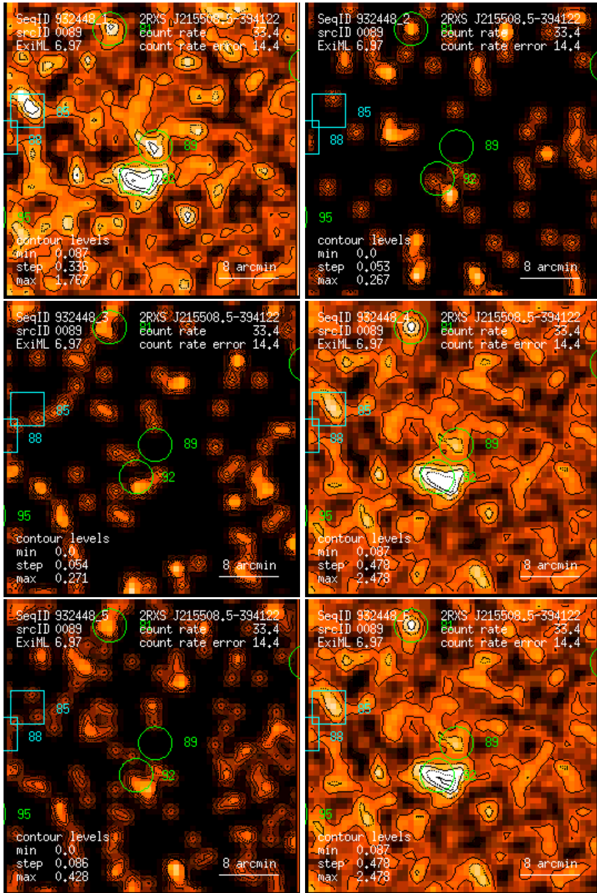
Figure 89: RASS 932448: detection 0089: band rate images, Gaussian filter: (1) PSPC channels 11 – 41, (2) 52 – 90, (3) 91 – 201, (4) 11 – 235, (5) 52 – 201, (6) 11 – 201. Broad band rates in counts/ks. Band rate contour levels in counts/ks/arcmin 2 .
