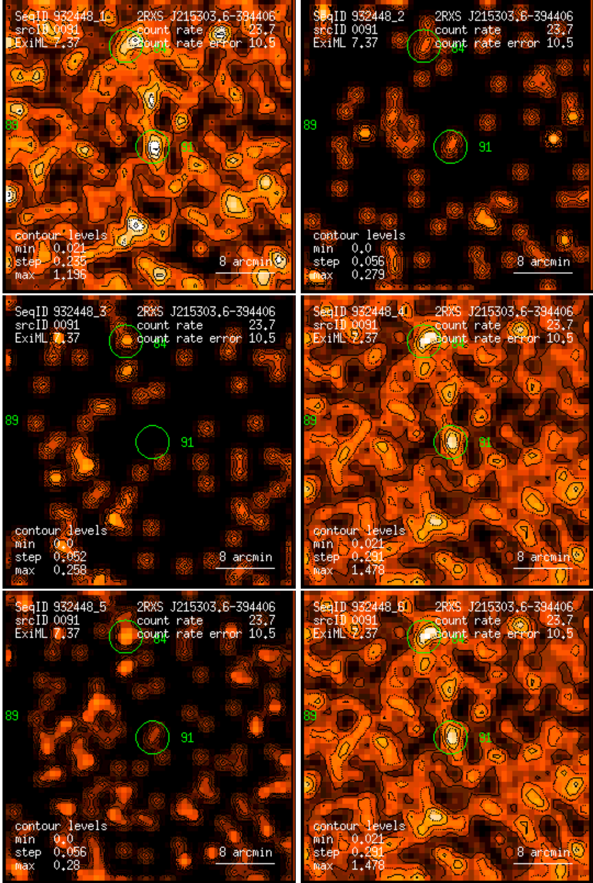
Figure 91: RASS 932448: detection 0091: band rate images, Gaussian filter: (1) PSPC channels 11 – 41, (2) 52 – 90, (3) 91 – 201, (4) 11 – 235, (5) 52 – 201, (6) 11 – 201. Broad band rates in counts/ks. Band rate contour levels in counts/ks/arcmin 2 .
