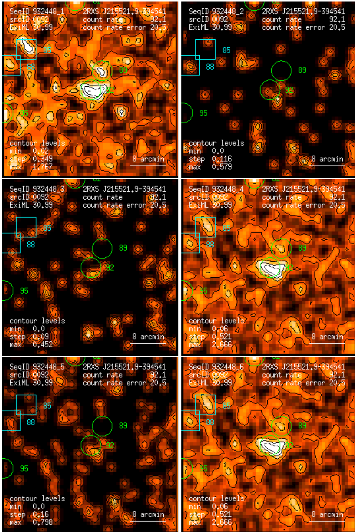
Figure 92: RASS 932448: detection 0092: band rate images, Gaussian filter: (1) PSPC channels 11 – 41, (2) 52 – 90, (3) 91 – 201, (4) 11 – 235, (5) 52 – 201, (6) 11 – 201. Broad band rates in counts/ks. Band rate contour levels in counts/ks/arcmin 2 .
